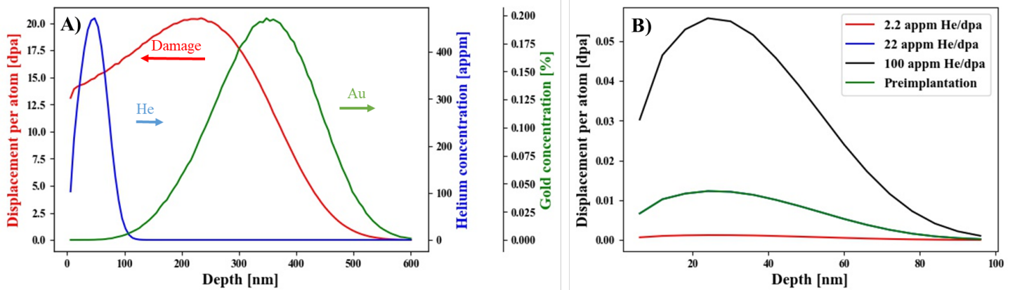
Figure 1: SRIM calculation for implantation depth into the HT9 samples by the 10 keV \text{He}^+ and 4 MeV \text{Au}^{2+} ions. A) shows the damage profile of the gold ions, the percentage gold and the
