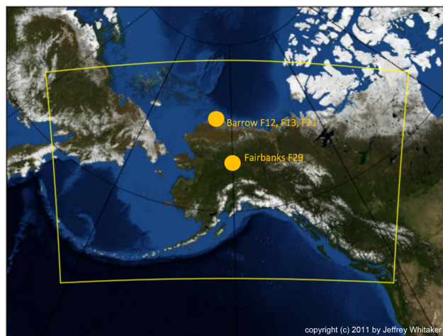
Figure 2. Model domain (yellow) used in this study centered over Fairbanks with a horizontal resolution of 10 km. The cities of Barrow (now Utqiagvik; 71.18° N, 156.44° E) and Fairbanks (64.83° N, 147.77° E) over which the F12, F13, F21 and F29 flights took place are also shown with orange dots.
