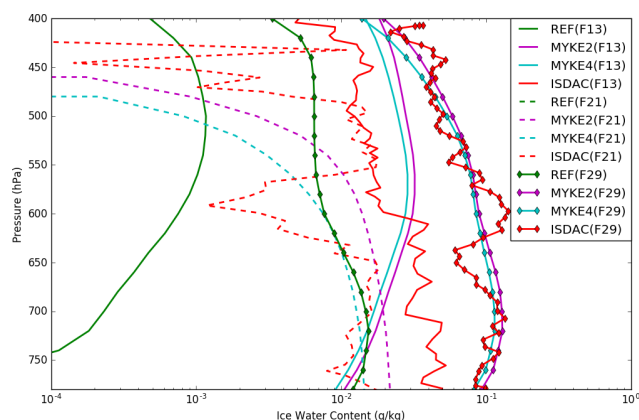
Figure 6. Comparison of the observed (red) and simulated (REF in green, MYKE2 in purple and MYKE4 in cyan) vertical profiles of IWC along flights F13 (solid lines), F21 (dashed lines) and F29 (solid line with diamond markers).
