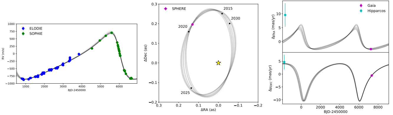
Fig. 2. Sample of 50 model orbits fitted on the HD 72946B data (colored points) from RV ( left ), imaging ( middle ), and astrometry ( right ). Middle panel: yellow star marks the location of the primary star, and the black dots show the median predicted position for given epochs.
