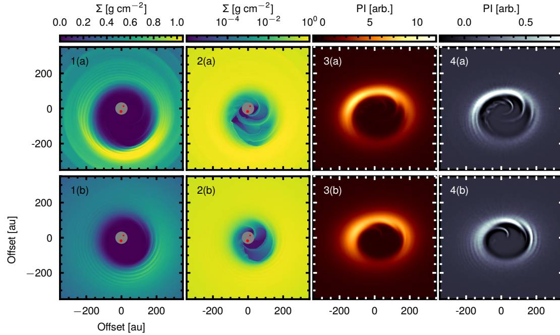
Fig. 8. Surface density output of our simulations in linear (left column; 1(a) and (b)) and logarithmic (center left column; 2(a) and (b)) color stretch. The center right column (3(a) and (b)) shows the simulated polarized intensity images evaluated at 1.67\,\mu\text{m} . This image was calculated after inclining and orienting the disk as in the observations. The right column (4(a) and (b)) shows the polarized intensity image of the center right column, processed with a high-pass filter. In each column, the panel in the first row (a) corresponds to the model with h=0.11 , the panel in the second row (b) to h=0.15 .
