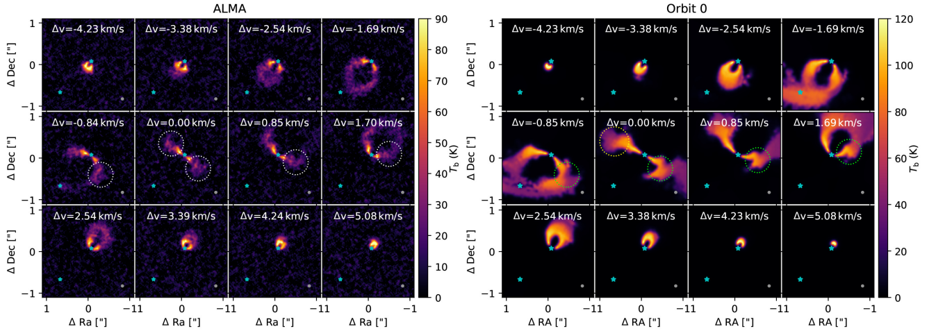
Figure 9. Channel maps of the ^{12}\text{CO } J=3-2 line. Left-hand panel: ALMA observations, right-hand panel: synthetic observations for orbit 0. The positions of both stars are marked in cyan and the beam is in the lower right-hand corner. The dotted circles show the locations of the kinks in the velocity field caused by the spirals in different channels. Velocities are relative to the systemic velocity of 5.12 \text{ km s}^{-1} .
