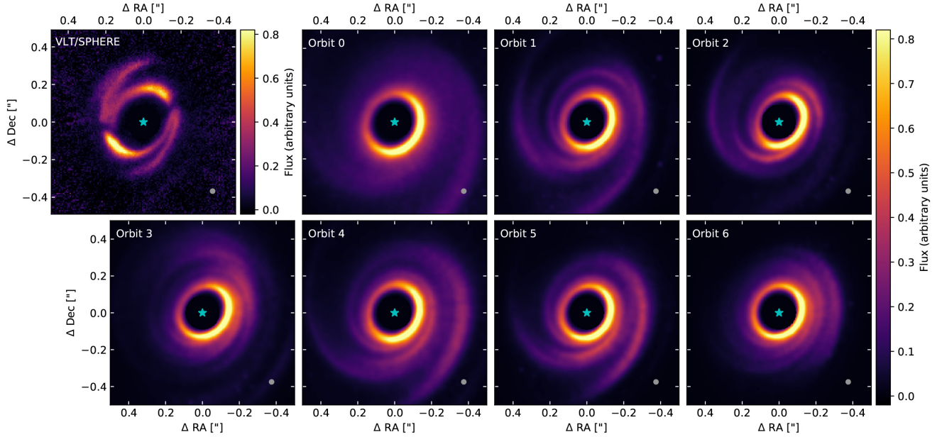
Figure 10. I' band scattered light images. Top left-hand panel: VLT/SPHERE observation from Benisty et al. (2017), then from left to right and top to bottom: synthetic observations for orbits 0 to 6. The synthetic images are convolved with a Gaussian beam of \theta = 24 mas (shown in the lower right-hand corner), and scaled by r^2 , the square of the distance to the central star. We added a 185 mas-diameter coronagraph mask to hide the emission from the central star (whose position is marked in cyan), as in the VLT/SPHERE observations. Note the difference in scale with Fig. 8.
