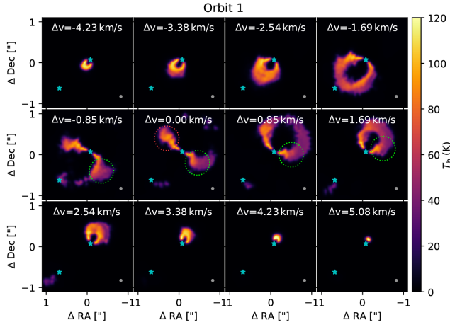
Figure A7. Synthetic channel maps of the ^{12}\text{CO } J=3-2 line for orbit 1. The positions of both stars are marked in cyan and the beam is in the lower right-hand corner. The dotted circles show the locations of the velocity kinks caused by the spirals in different channels.
