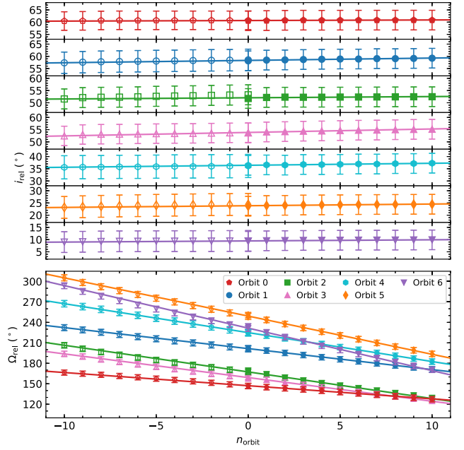
Figure 5. Evolution of the relative tilt and twist angles for the seven orbital configurations in the rewind simulations (open symbols) compared to the forward (filled symbols) ones. The solid lines are linear fits to the values in the forward simulations.
