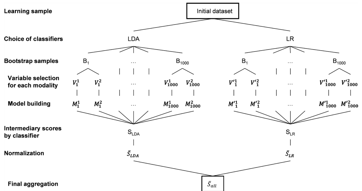
Figure 1. Methodology of construction of the ensemble score.
