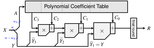
Fig. 2. A fixed-point polynomial evaluator, using uniform segmentation and a Horner scheme with truncated multipliers – see [14] for more details.
