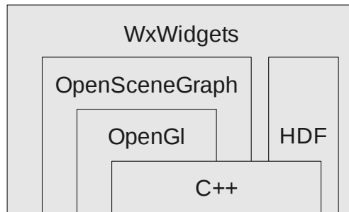
Fig. 8. GIDE Architecture
