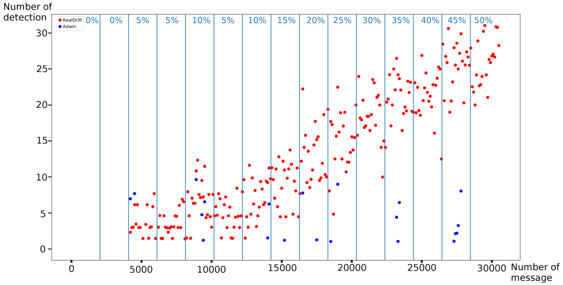
Fig. 5: Detection of ADWIN algorithm for pothole scenario
