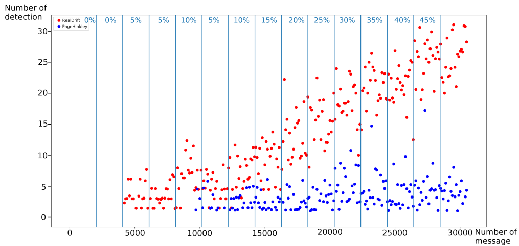
Fig. 3: Detection of Page-Hinkley algorithm for pothole scenario
