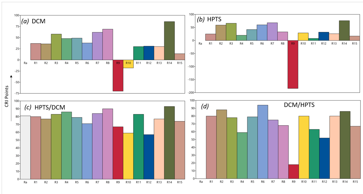
Figure 8: R-values charts for films containing: (a) DCM, (b) HPTS, (c) HPTS over DCM and (d) DCM over HPTS; measured under 450 nm LED illumination (440 mA, 3 V). All the films were placed in a remote-phosphor configuration at 0.3 cm from the LED chip.
