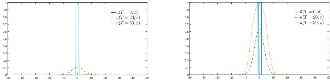
Figure 1: The graphs shows the influence of the distribution at time T = 0 . On the left hand side the initial population u(0, x) is concentrated into a single block of mass m = 2.22 , it means that the whole population was released at the same spot. Also is showed the resulting distribution after different times laps: clearly the infected population tends to disappear as time goes by.
