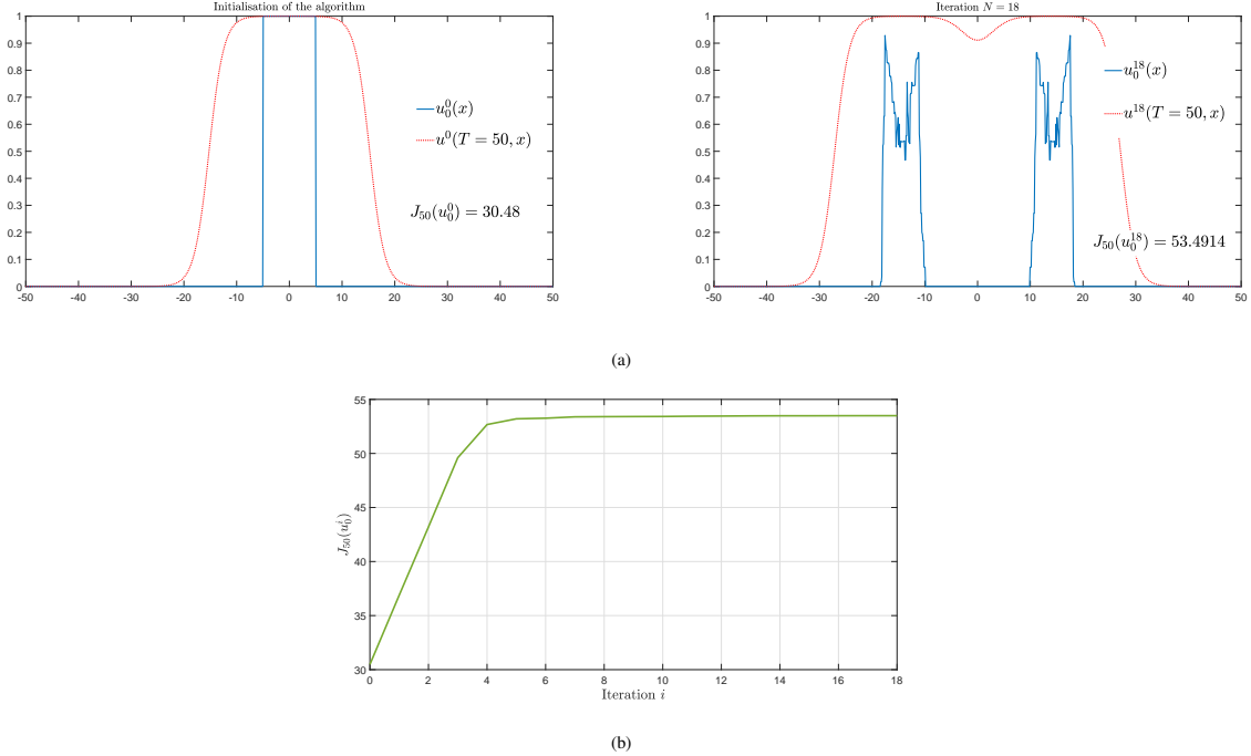
Figure 3: Considering a fixed mass L = 10 , this figure shows the initial data associated with the first and the last iteration of the algorithm and the corresponding solutions of eq. (1.2) (a). We also show the evolution line of the operator J_{50}(u_0^i) from the first iteration to the last one (b). Note that the limit reached after 18 iterations is an initial data separated in two blocs and shows singularities as a consequence of the definition of the initial solution within the set \Omega_{p,\lambda^{18}} .
