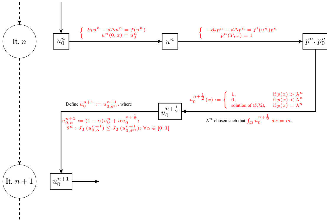
Figure 2: Scheme of the numeric algorithm.
