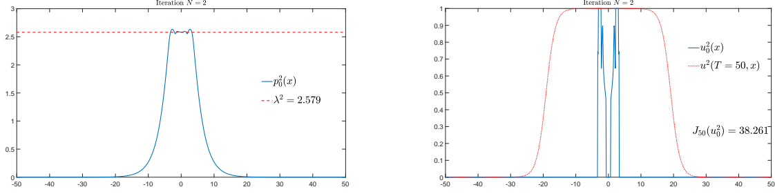
Figure 4: The figure correspond to the 2^{nd} and also last iteration of the algorithm for a given final time T = 50 and a fixed mass L = 4 . At the left hand side we show the adjoint state p which is the solution of the equation (5.70) and its associated value \lambda^2 mentioned in Theorem 1. Note that in this case the set \Omega_{p, \lambda^2} is not negligible so the associated u_0^2 showed at the right side present singularities arising from the solution of (5.72) within this set.
