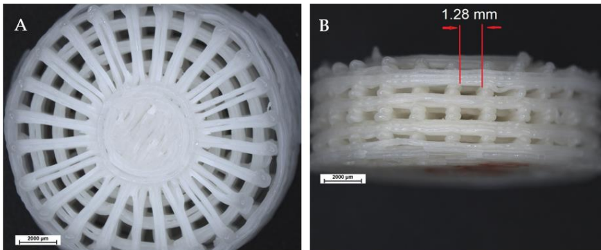
Figure 7. A representative bi-layer sample from the top (A) and side (B) views.
