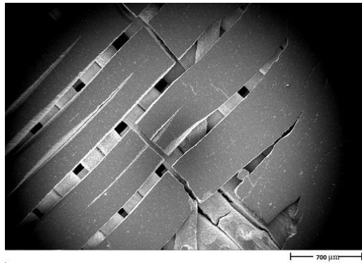
Figure 6. Low magnification SEM image of a dense sample illustrating open spaces between filaments.
