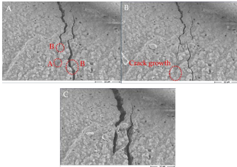
Figure 12. Cracks propagations through the microstructure of a porous sample (in opposite direction) under compressive loading taken by ESEM.
