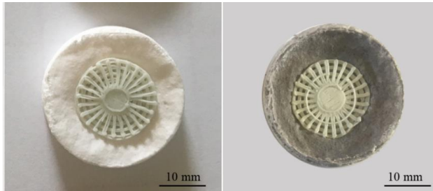
Figure 14. Digital photographs of two representative hybrid ceramic polymer samples. Left: Ag + -free PCL/BCP layer; right: Ag + -added PCL/BCP layer.
