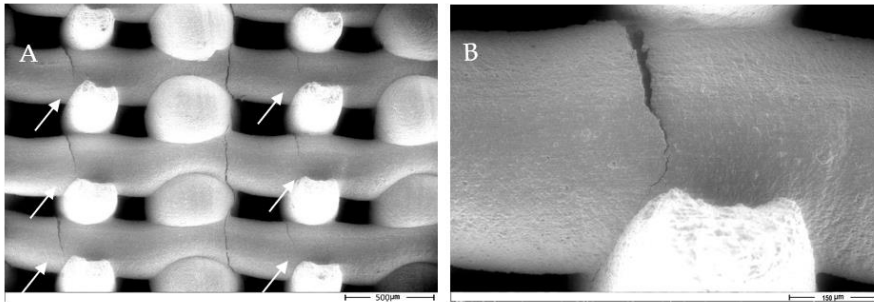
Figure 10. Longitudinal cracks running through the structure of a porous scaffold during the compression test observed by ESEM.
