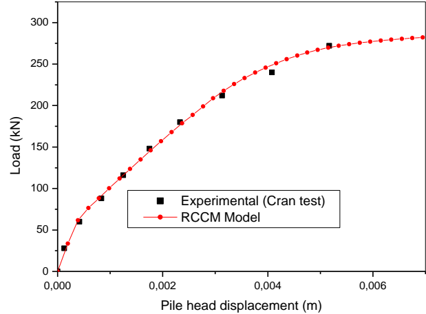
Fig. 6: Simulation of the Cran test
