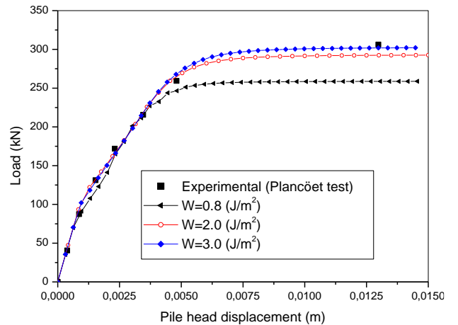
Fig. 8 : Influence of the decohesion energy ( w )
