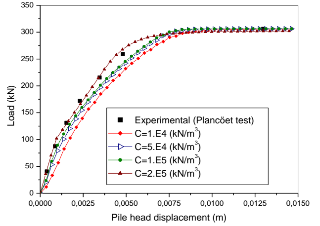
Fig. 7 : Influence of the initial stiffness C_n, C_t
