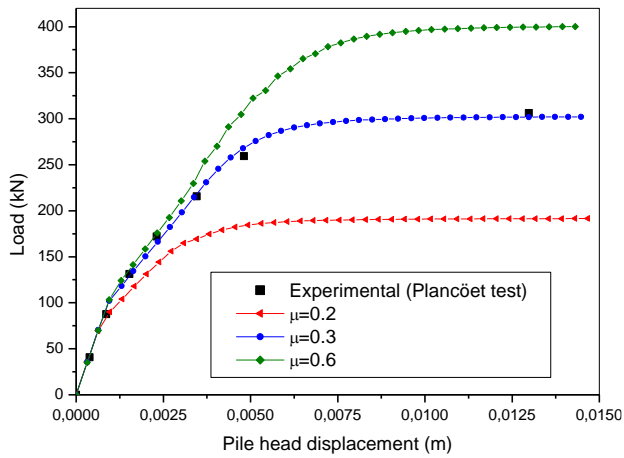
Fig. 9 : Influence of the friction coefficient \mu (for \alpha = 0 )
