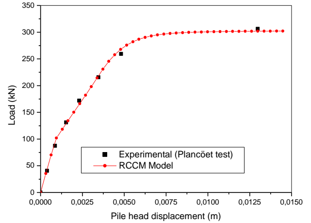
Fig. 5: Simulation of the Plancötet test
