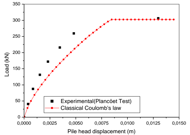
Fig 4: Results with classical Coulomb's law
