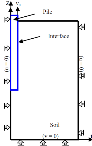
Fig. 2. Geometry and boundary conditions
