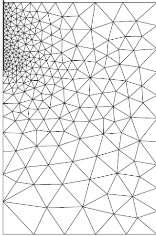
Fig. 3: Finite element mesh
