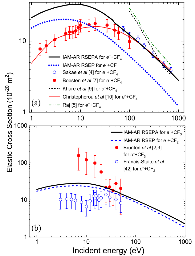
Fig. 1. Elastic integral cross sections of electron scattering by CF and \text{CF}_4 (a) as well as by \text{CF}_2 and \text{CF}_3 (b) molecules.
