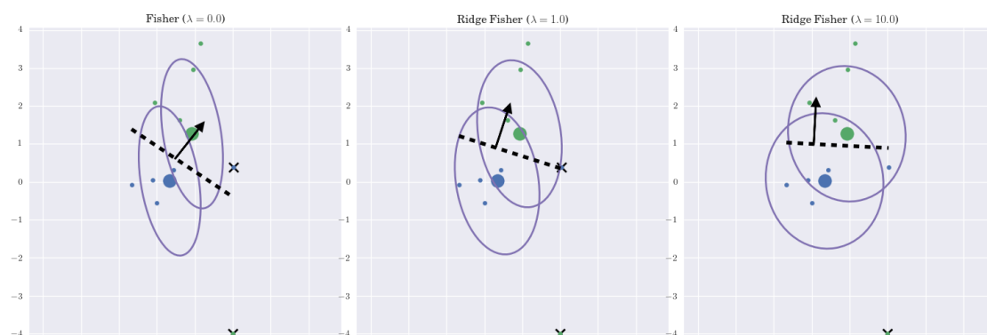
Fig. 9: The Ridge Fisher most discriminant projection
