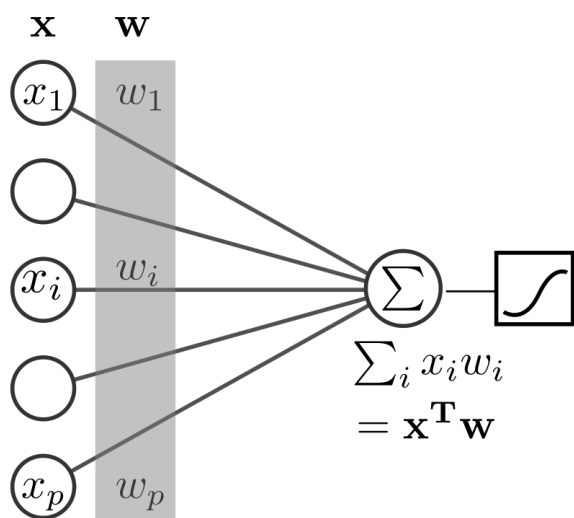
Input of size p Weights Output of size 1 Activation function [width=15cm]
