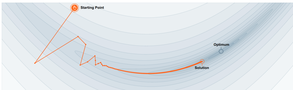
Fig. 5: With momentum: accumulate velocity to avoid oscillations
