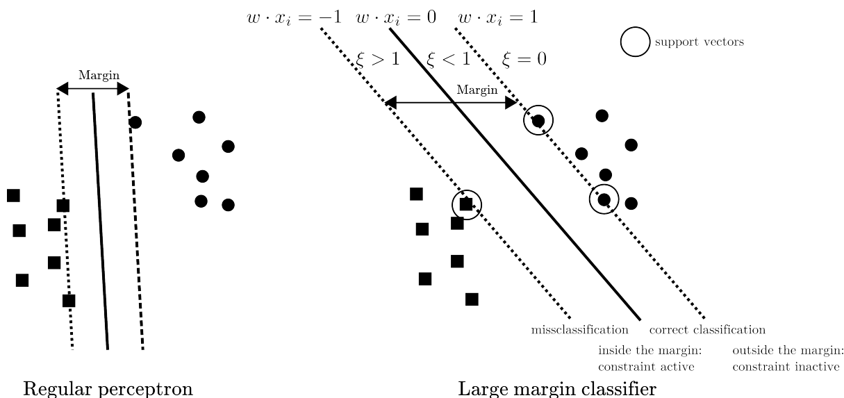
Fig. 10: Linear lar margin classifiers
