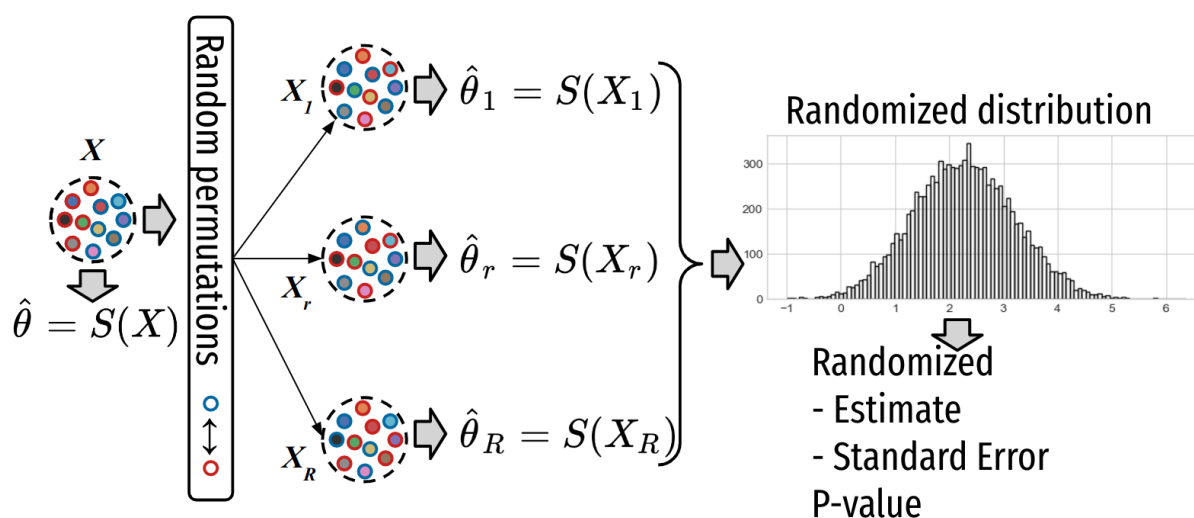
Fig. 5: Bootstrapping procedure
