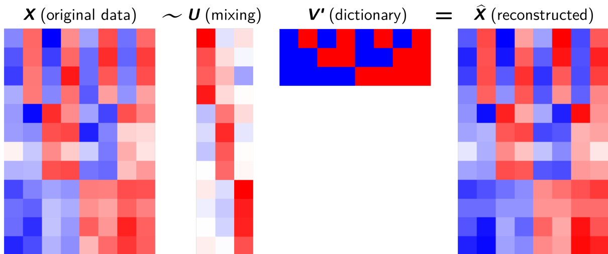
Fig. 1: Matrix factorization
