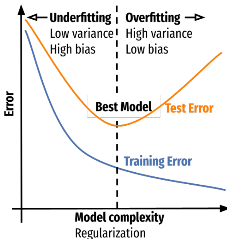
Fig. 1: Model complexity
