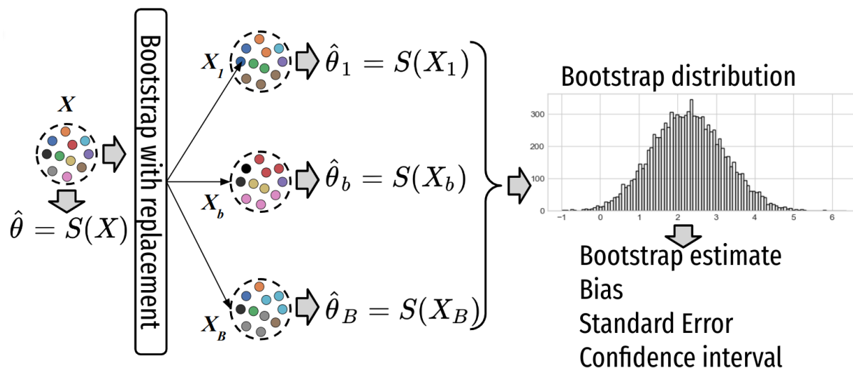
Fig. 6: Bootstrapping procedure
