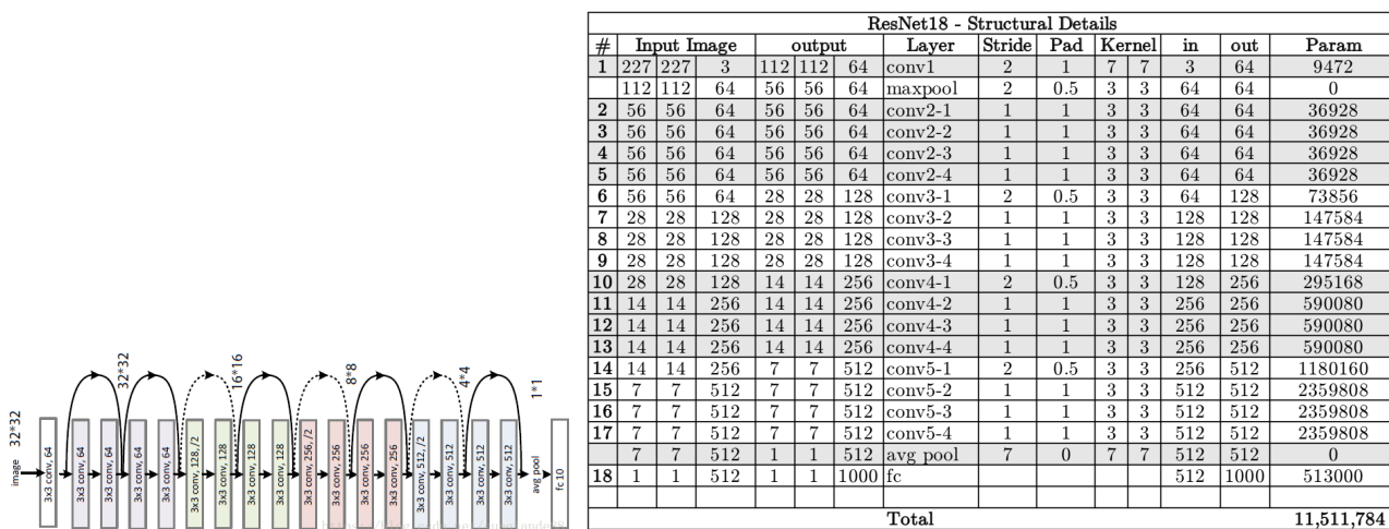
Fig. 3: ResNet block
