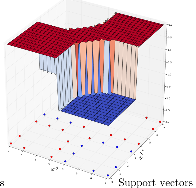
Fig. 12: Support Vector Machines.
