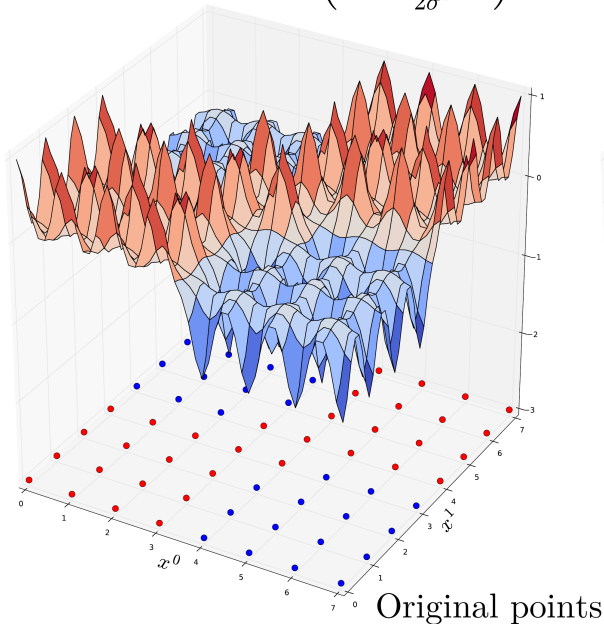
Fig. 12: Support Vector Machines.
