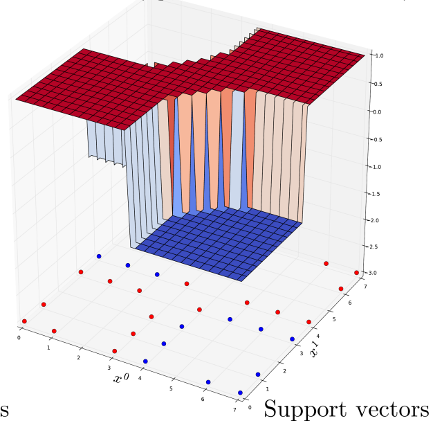
Fig. 12: Support Vector Machines.
