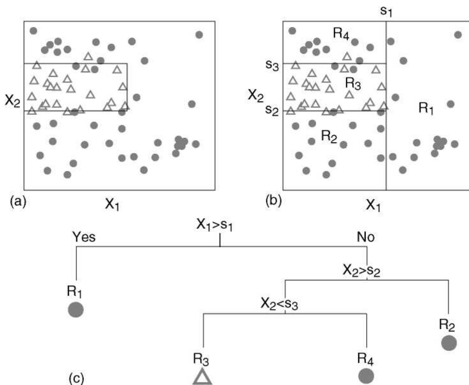
Fig. 13: Classification tree.
