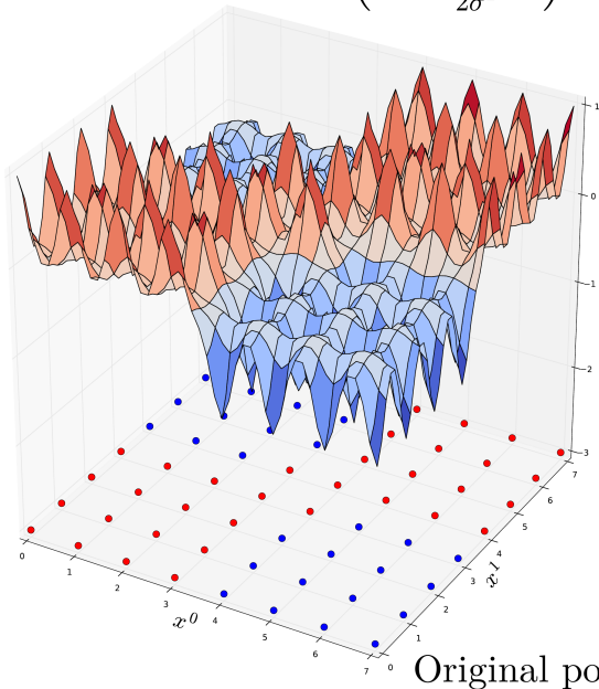
Fig. 12: Support Vector Machines.
