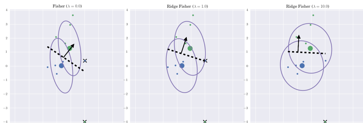
Fig. 10: The Ridge Fisher most discriminant projection
