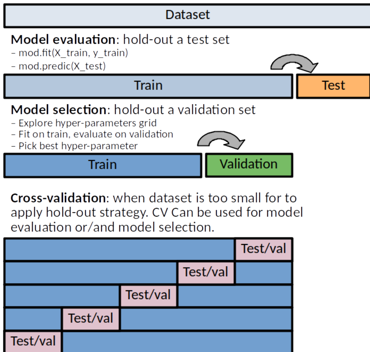
Fig. 14: Train, validation and test sets.
