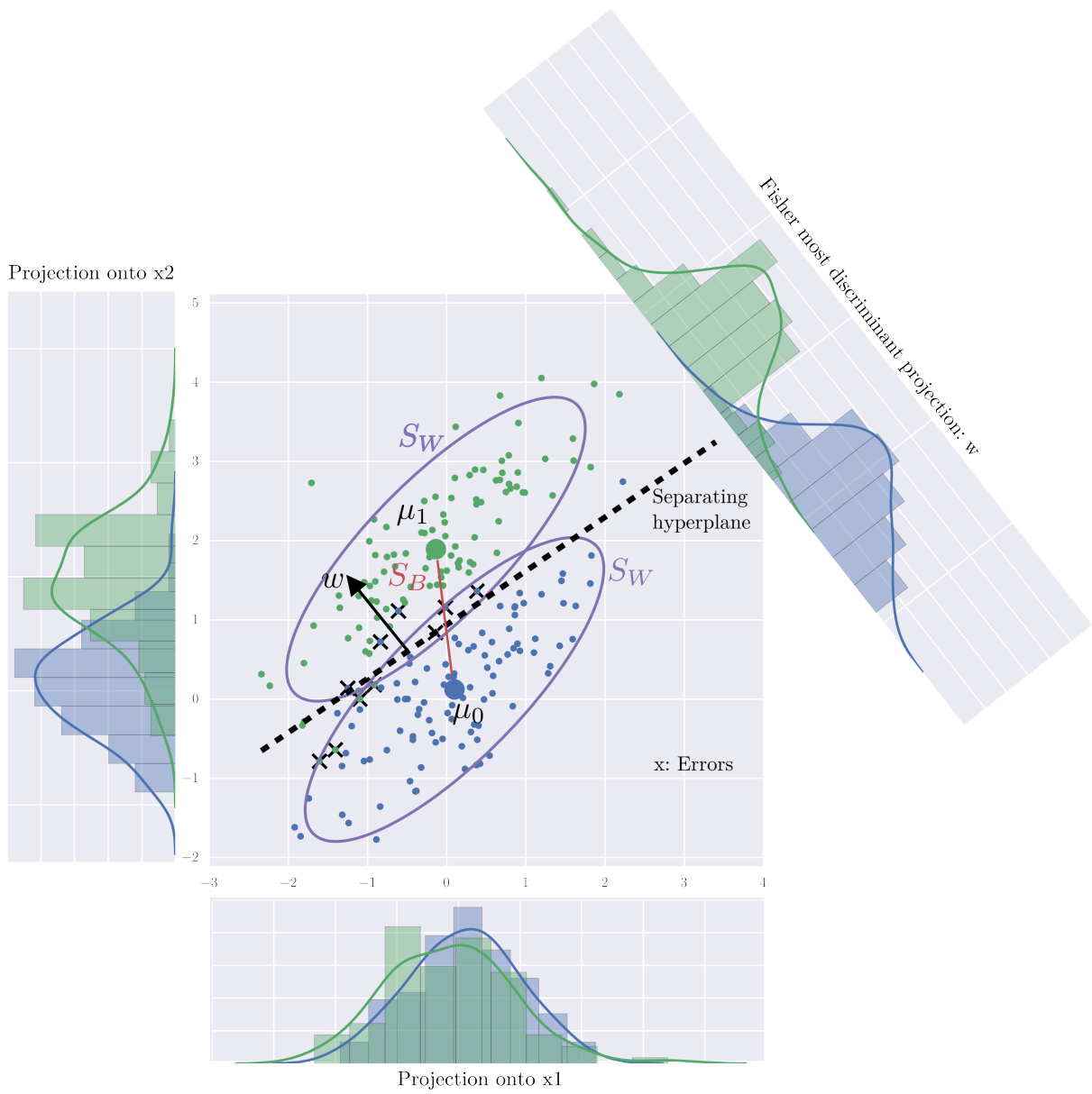
Fig. 8: The Fisher most discriminant projection
