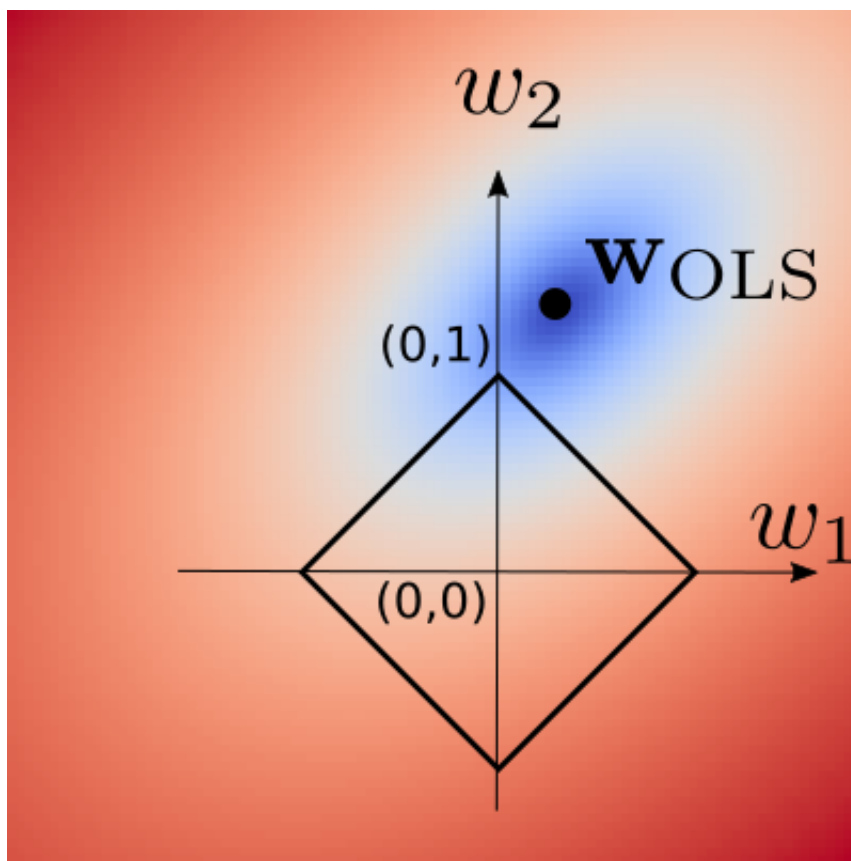
Fig. 4: Sparsity of L1 norm
