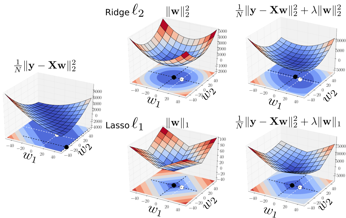
Fig. 5: l_1 and l_2 shrinkages
