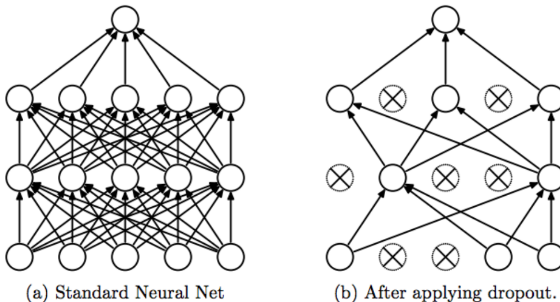
Fig. 4: Dropout
