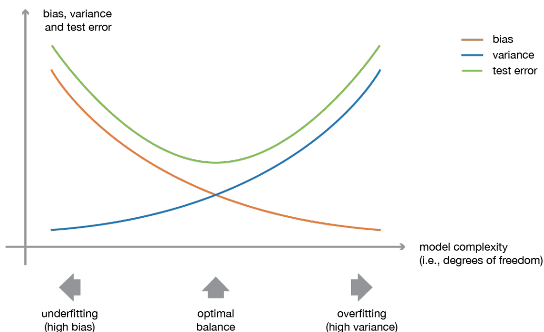
Fig. 15: towardsdatascience blog
