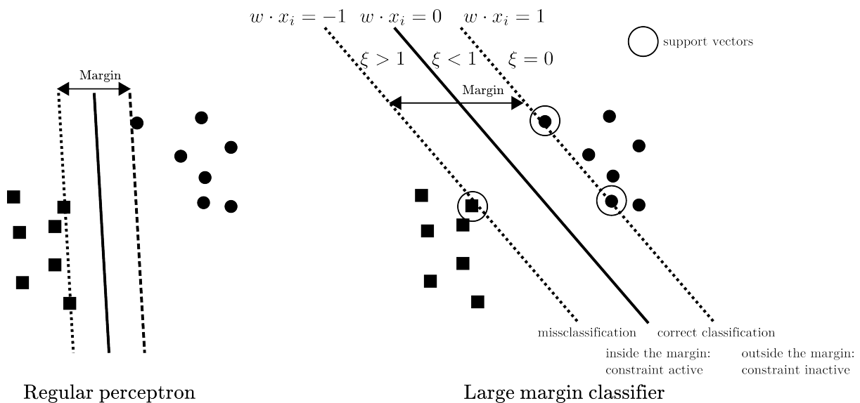
Fig. 11: Linear lar margin classifiers
