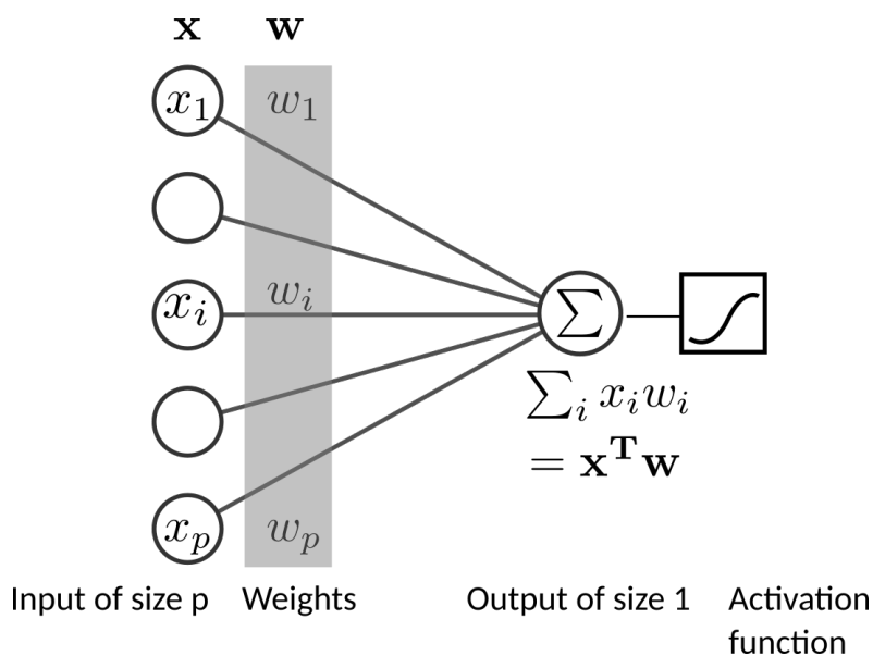
Fig. 7: Linear (logistic) classification
