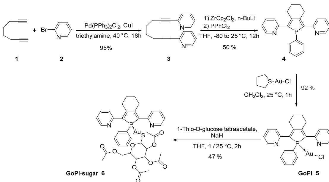
Scheme 1. Synthetic route to prepare 1-thio- \beta -D-glucopyranose 2,3,4,6-tetraacetato-S-Au{1-phenyl-2,5-di(2-pyridyl)phosphole} (GoPI-sugar).
