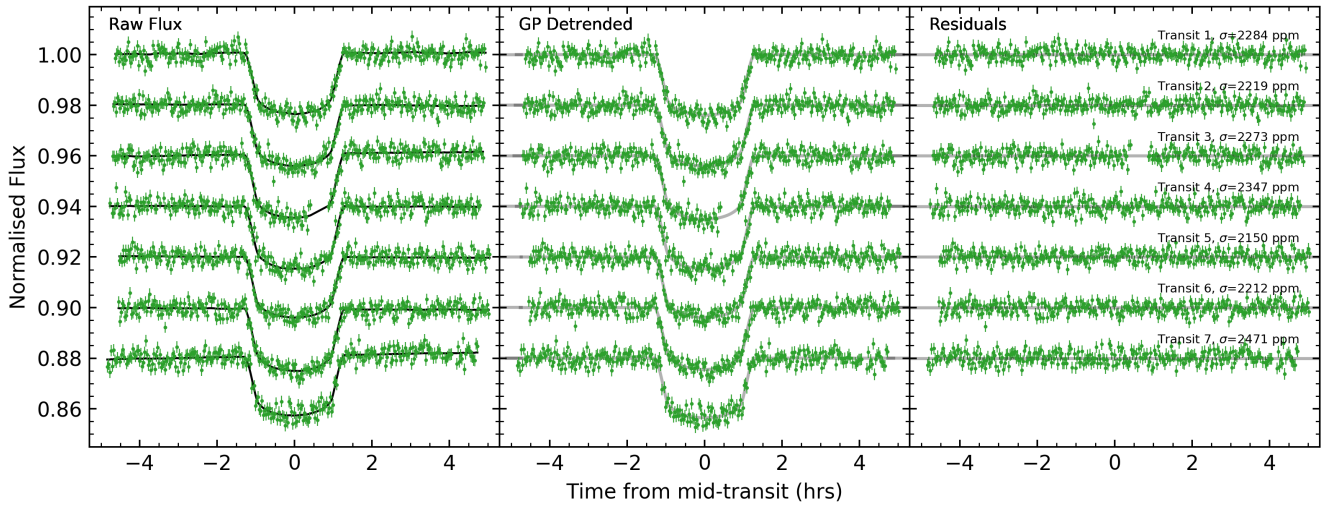
Figure 3. Normalised TESS photometric light curves multiplied by an arbitrary constant. Left: Raw extracted light curves with black lines indicating the GP transit plus systematic model fits. Centre: Light curves after removal of GP systematic component. The best fitting transit models from Mandel & Agol (2002) are displayed in grey. Right: Residuals after subtraction of best fitting models from the GP systematic corrected light curves.
