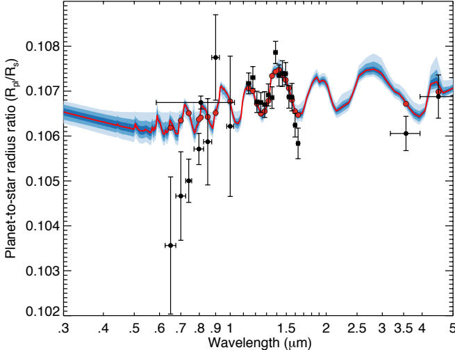
Figure 12. Atmospheric spectrum from chemical equilibrium ATMO retrieval based on HST, LDSS, TESS, and Spitzer transit depth estimates. The red line shows the best-fit model, and the blue areas indicate the 1, 2, and 3\sigma uncertainties. Due to the high cloud deck that the model is driven to by the opacity at \sim 1\mu\text{m} , this model does not fit the decreased absorption at 1.6\mu\text{m} or the positive slope in the bluer wavelengths. This model had a BIC of 70.75 for 25 data points and 8 free parameters.
