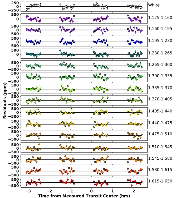
Figure 3. White and spectroscopic residuals for light curves extracted from the HST/WFC3 data. Values represent 1\sigma residuals.
