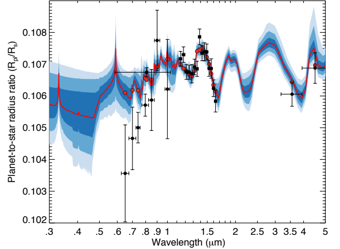
Figure 13. Atmospheric spectrum from ATMO free-chemistry retrieval based on HST, LDSS, TESS, and Spitzer transit depth estimates. The red line shows the best-fit model. With the FeH and \text{H}^- , this model better accommodates the slope of the water feature at longer wavelengths as well as the diminished opacity in the bluer wavelengths. This model also accommodates a clearer atmosphere than the chemical equilibrium model, as well as a higher temperature ( \sim 1200\text{ K} ). This model had a BIC of 60.75 for 25 data points and 8 free parameters.
