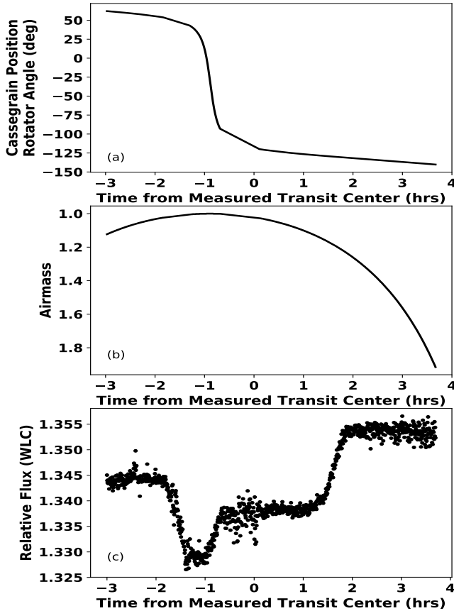
Figure 4. (a) The Cassegrain Position Rotator Angle as a function of time for the white light curve (WLC) transit extraction. Note that the telescope passed through zenith, as indicated by both the telescope position and the airmass (b). This resulted in a shift of the illumination on the detector and an associated shift in the relative flux between the target and reference stars, as shown in (c).
