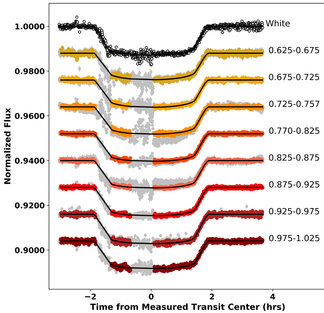
Figure 7. WASP-79b white and spectroscopic light curves extracted from December 2016 LDSS-3C data using the fitting process described in Stevenson et al. (2016a) . As with the WFC3 data, the results are binned and normalized to the system flux, and the error bars represent 1\sigma uncertainties. The black lines show the best-fit models, and the wavelength range for each of the 8 channels is specified in \mu\text{m} ( Stevenson et al. 2016a ). The grey points represent the original data, and the colored points represent the data that were retained from the noise and outlier masking process.
