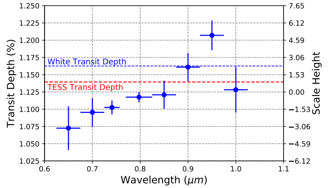
Figure 10. Spectrum constructed from transit depths of 8 wavelength bins of LDSS-3C data. The large spread in transit depth estimates - particularly noticeable at 0.9 and 0.95 \mu\text{m} - is likely due to interference from Earth’s atmosphere that could not be fully accounted for due to the distance of the reference star from the target star. The 0.65 \mu\text{m} point may be low due to detector cutoff at the blue edge. The transit depth estimates for the white light curve analysis described in 2.3.2 and for the TESS analysis (Section 2.1) are provided for comparison.
