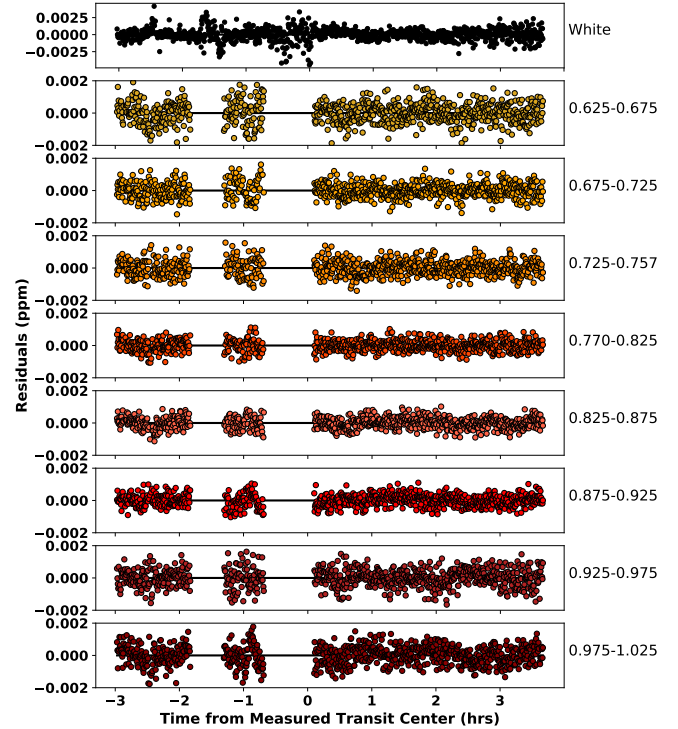
Figure 8. White and spectroscopic residuals for the light curves extracted from the LDSS-3C data. Values represent 1\sigma residuals. The gaps in the spectroscopic plots indicate times for which noisy observation data were masked.
