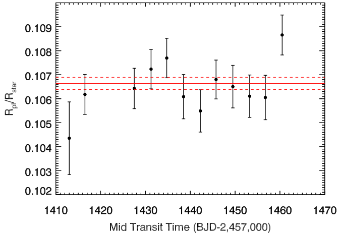
Figure 1. Transit depth estimates for the 12 transits of WASP-79b available from TESS. Estimates are shown with 1\sigma uncertainties. The red lines indicate the weighted mean of the transit depths with 1\sigma uncertainties.
