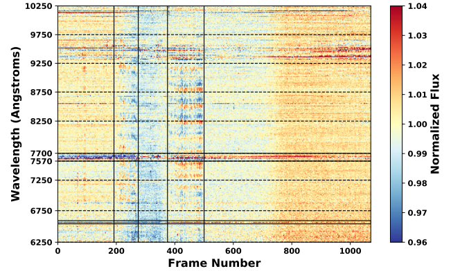
Figure 5. Two-dimensional light curve for the Dec 2016 LDSS-3C WASP-79b observations showing the flux of the target star normalized against the flux of the reference star. Normalized flux is shown per wavelength as a function of frame number. The 6540-6590, 7570-7700, and 9250-9750 channels show increased absorption, particularly early on in the observation. The 6540-6590 and 7570-7700 channels were masked to remove their influence from the light curve extraction. The solid vertical lines indicate the times for which data was removed based on visual inspection as described in Step 1 of the iterative outlier rejection process.
