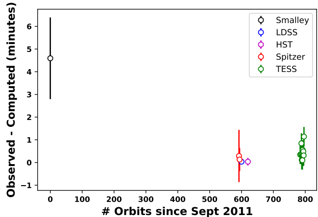
Figure 11. Comparison of observed transit times with computed transit times for Smalley, WFC3, LDSS-3C, Spitzer, and TESS observations. Computed transit times are based on the updated ephemeris and orbital period provided in Table 2.
