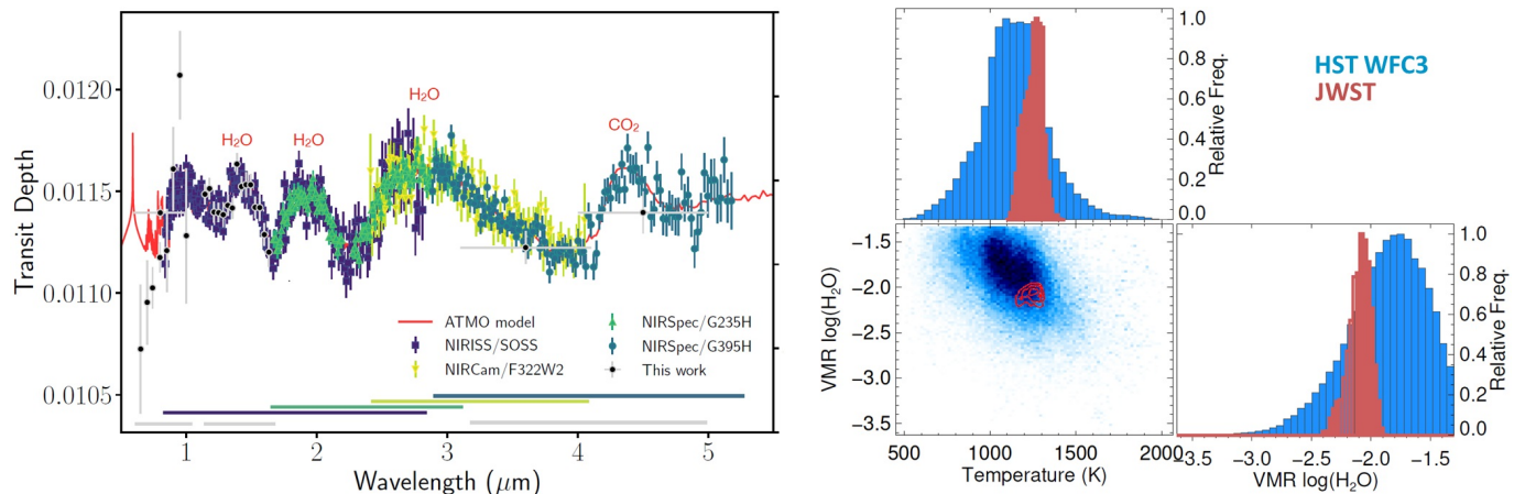
Figure 16. JWST simulated observations (left) and anticipated temperature and water constraints (right) from the PanCET Program observations of WASP-79b. Left: the simulated observations were generated using Pandexo (Batalha et al. 2017), based on the free-chemistry atmospheric retrieval spectrum and the observation data described previously. Simulated observations are shown with the estimated LDSS, TESS, HST, and Spitzer transit depths. Results are binned to R = 100 (left). The LDSS-3 data constrain the scattering slope, compared to Figure 7 in Bean et al. (2018), which shows the Pandexo results for the best-fit solution for just the HST/WFC3 data with contributions from haze scattering. Right: anticipated constraints (red) on the atmospheric temperature and water abundance compared with constraints from HST (blue). The constraints are improved by orders-of-magnitude due to increased data resolution and the presence of multiple water features (Greene et al. 2016).
