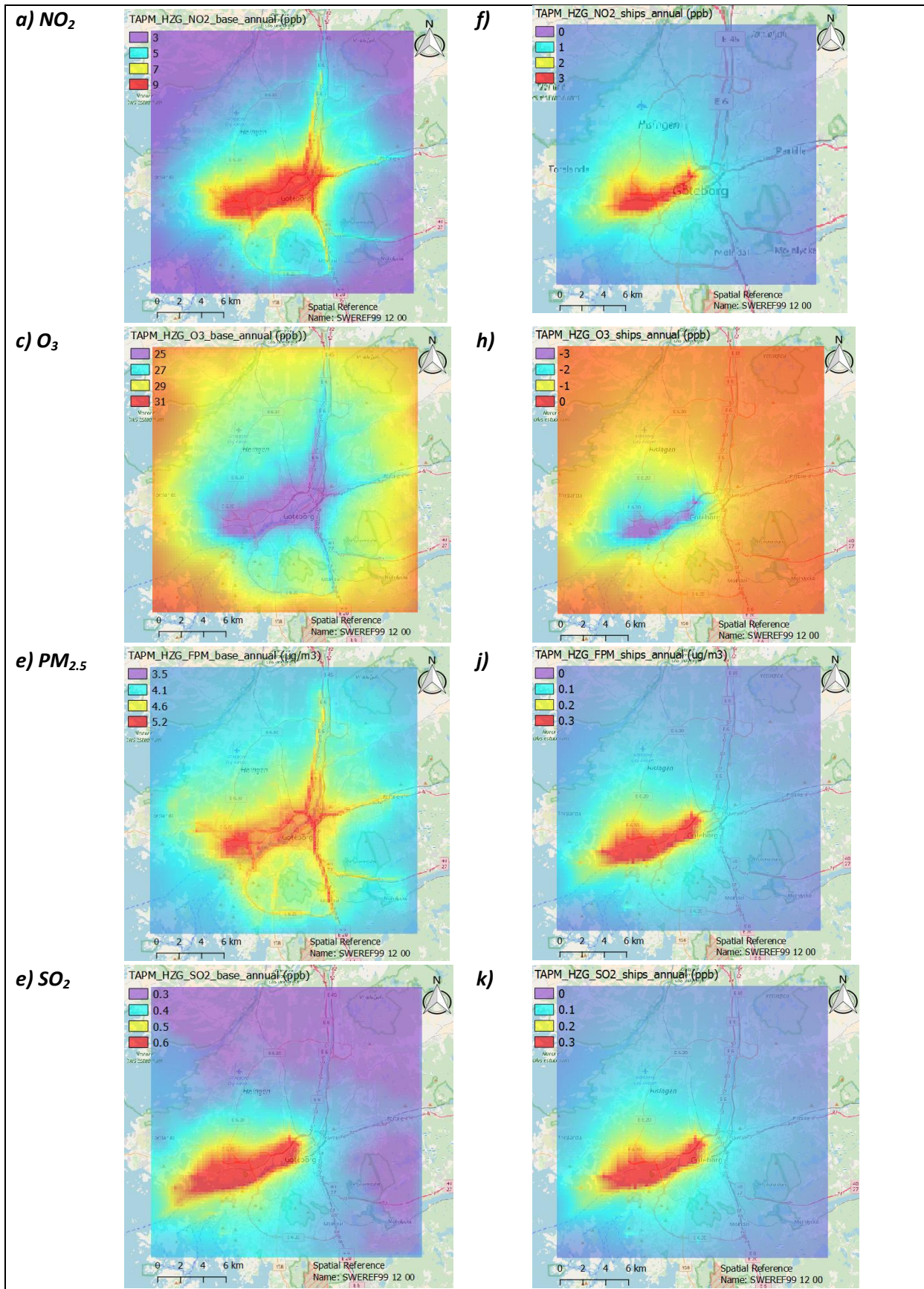
Figure 11: Annual mean values of NO 2 , O 3 , PM 2.5 and SO 2 in the city of Gothenburg from TAPM by HZG. Total concentrations including all sources are displayed on the left side, the contribution from shipping is given on the right side.
