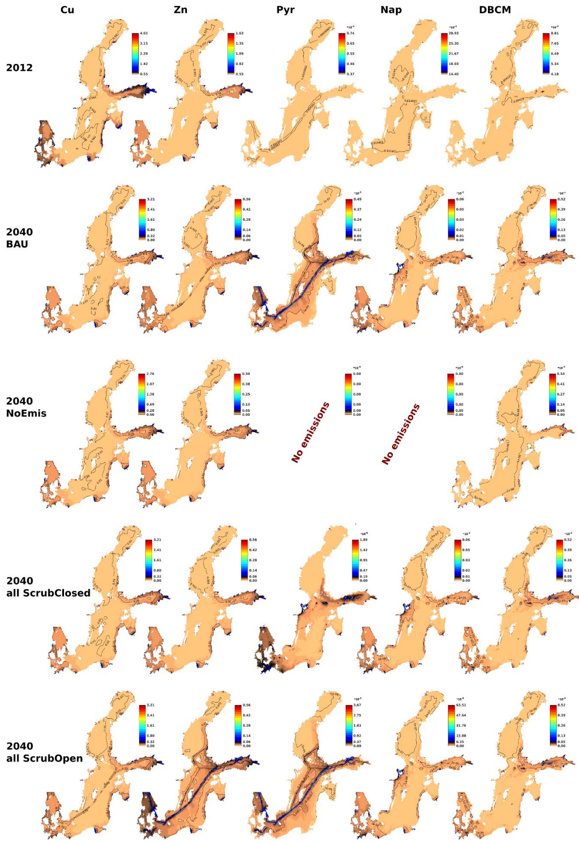
Figure 20 Maps of the Baltic Sea showing the concentrations of copper (Cu), zinc (Zn), pyrene (Pyr), naphthalene (Nap) and dibromochloromethane (DBCM), resulting from the emissions in the reference year 2012 (2012), and the scenarios Business as usual 2040 (2040 BAU), Zero emissions to water 2040 (2040 NoEmis) and Scrubber 2040 all closed (2040 all ScrubClosed). The colour bars represents concentration in µg/L, and the lines with numbers in the sea areas depicts areas with the concentration given by the corresponding number. The missing maps for pyrene and naphthalene indicates that these compounds would have no emissions under these scenarios.
