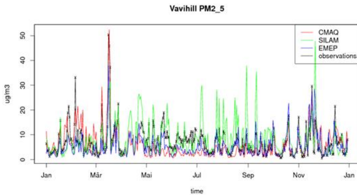
Figure S 5: Comparison of the modelled PM2.5 concentrations from CMAQ, SILAM and EMEP for the year 2012 with observations at Vavihill, South Sweden and Aspveten, East Sweden.
