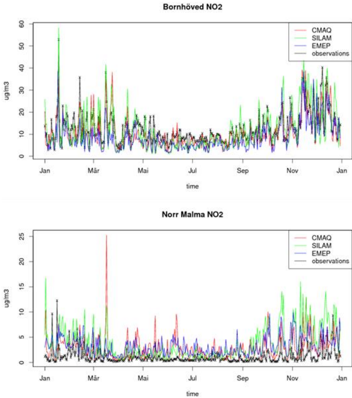
Figure S 4: Comparison of the modelled NO 2 concentrations from CMAQ, SILAM and EMEP for the year 2012 with observations at Bornhöved, Germany and Norr Malma, Sweden.
