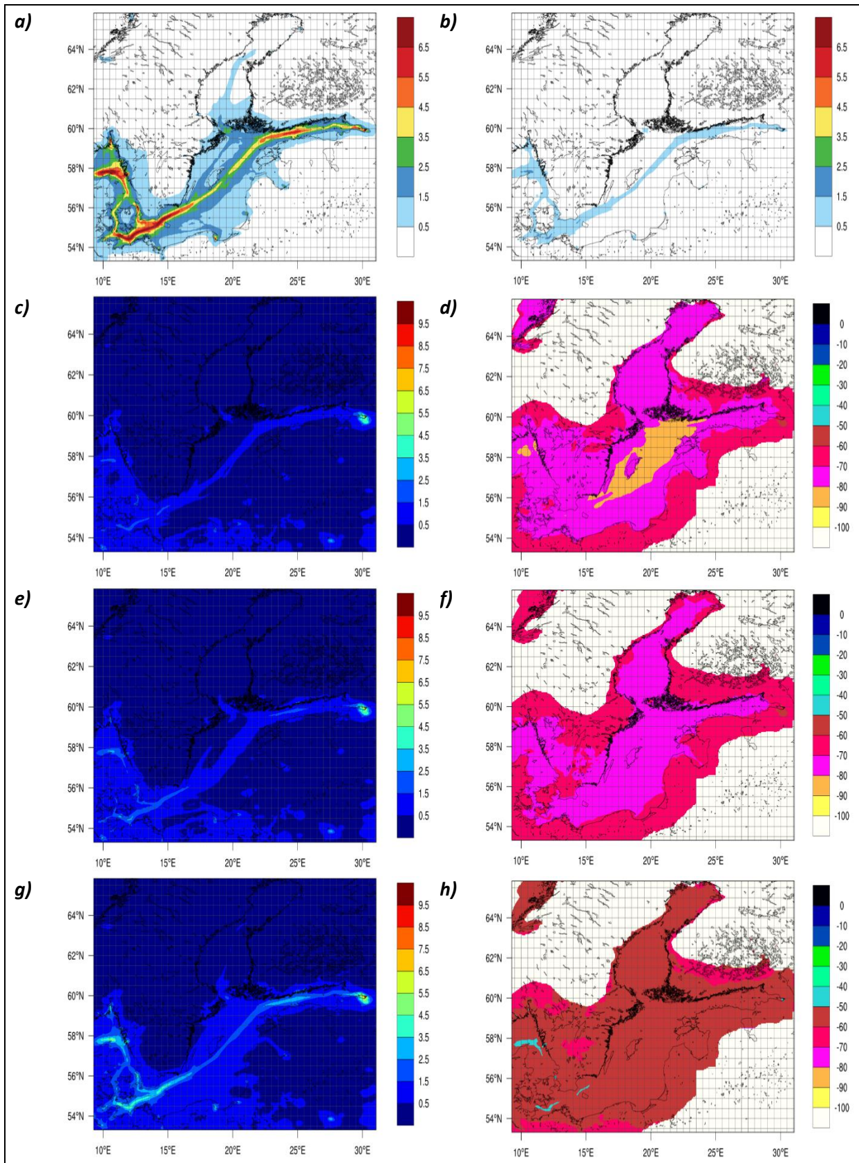
Figure 9: Air concentration of NO 2 as mean of summer months, JJA (unit: ppbV): future changes in the Baltic Sea region compared to present-day (2012) for three future scenarios. (a) Present-day ship contribution, (b) BAU scenario (2040) future ship contribution, (c) BAU scenario (2040) future situation, (d) relative change (%) of BAU scenario (2040) compared to present-day, (e) EEDI scenario (2040) future situation, (f) relative change (%) of EEDI scenario (2040) compared to present-day, (g) NoNECA scenario (2040) future situation, (h) relative change (%) of NoNECA scenario (2040) compared to present-day.
