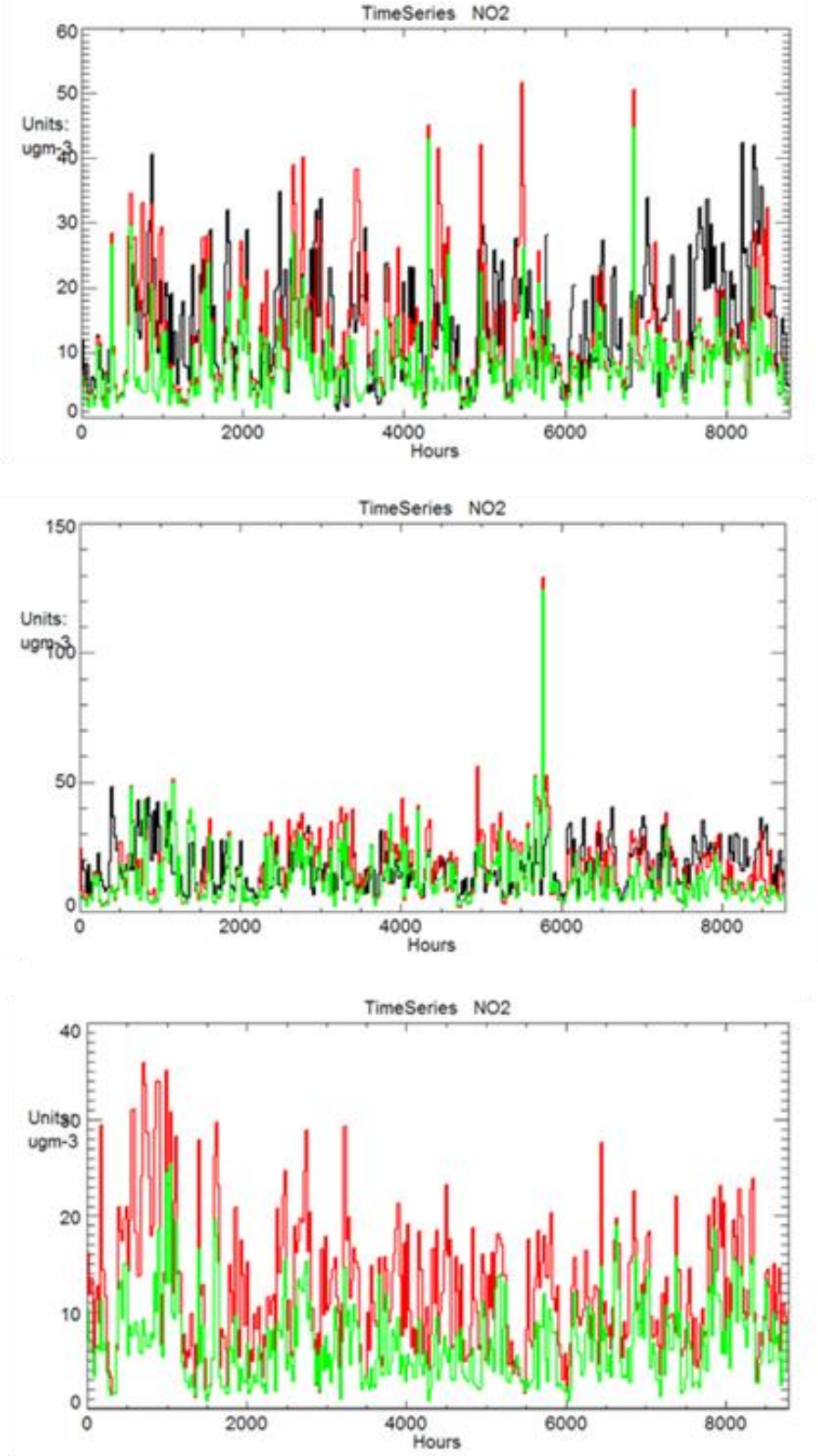
Figure S 6: Modelled time Series of NO2 concentrations at Rostock Warnemünde, Gdansk Noviport and Riga Vecmilgravis in 2012. Displayed are the simulations including all sources (red) and without ships (green). Observations are shown for comparison in black for Rostock and Gdansk.
