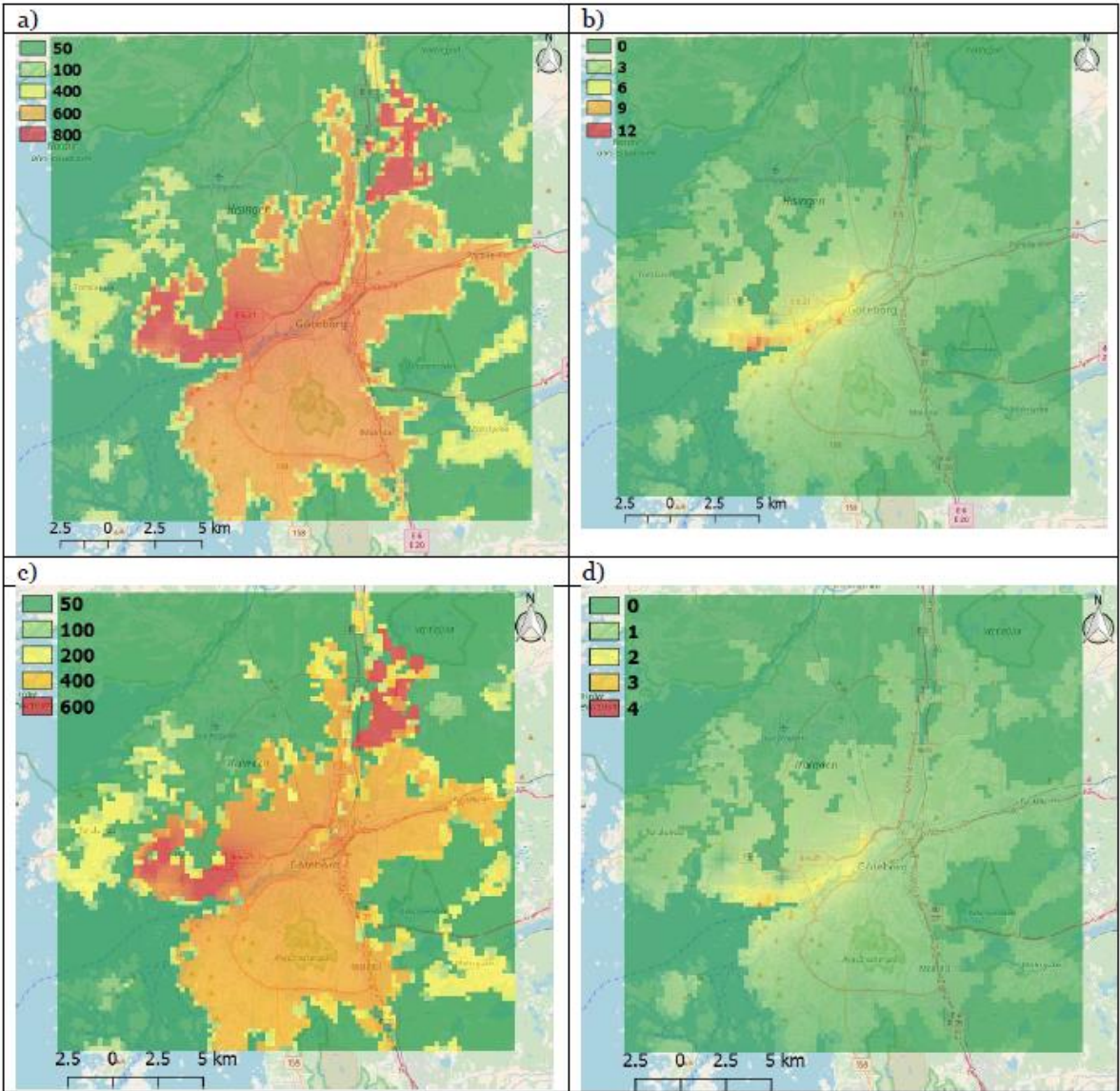
Figure S7: Exposure to PM2.5 concentrations of the population in Gothenburg in 2012 (a,b) and in 2040, BAU scenario (c,d). The total exposure in \mu\text{g}\cdot\text{m}^{-3}\cdot\text{capita}/\text{grid square} is shown on the left (a and c), relative contribution of the local shipping to the total exposure (in %) on the right (b and d).
