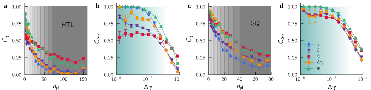
FIG. 7. Decay and growth correlation of the LJ data. Correlation decay C_\gamma = C(0, \gamma_{pl}(n_{pl})) between a structural field computed at \gamma_0 and plastic events occurring at strain \gamma . Correlation growth C_{\Delta\gamma} = C(\gamma_{pl} - \Delta\gamma, \gamma_{pl}) between a structural field \Delta\gamma away from a plastic event located at \gamma_{pl} . Results are for (HTL) ductile glasses (a-b) and (GQ) well annealed glasses (c-d). The different colors and symbols corresponds to the structural indicators labeled in (d). The gray gradient in (a) and (c) indicates the change in strain from \gamma_0 = 0 (transparent) to \gamma_{\text{yielding}} \simeq 7\% (opaque).
