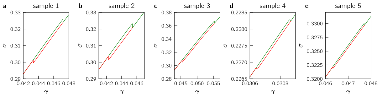
FIG. 3. Anelastic events. (a-e) Stress-strain curve around the first plastic event in 5 very stable glasses. The Green and red curves are the loading and unloading, respectively.
