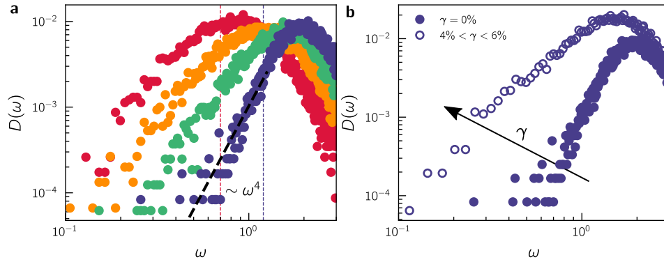
FIG. 8. Soft excitations. (a) Density of state of non-linear excitations in glasses prepared by SWAP. The black dashed line indicates the scaling D(\omega) \sim \omega^4 . The vertical colored lines indicate the frequency threshold used to define low-energy excitations, \omega^* = 0.7 and \omega^* = 1.2 for the most ductile T_{\text{ini}} = 0.3 and least ductile T_{\text{ini}} = 0.05 glasses, respectively. (b) D(\omega) for a finite \gamma ( 4\% < \gamma < 6\% ), comparing with \gamma = 0\% , for T_{\text{ini}} = 0.05 .
