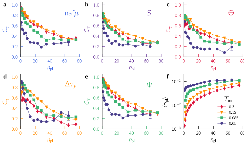
FIG. 5. Decay correlation and plastic activity. (a-e) Decay correlation C_\gamma = C(0, \gamma_{pl}(n_{pl})) for various indicators and glass stabilities. (f) Average plastic strain \langle \gamma_{pl} \rangle as a function of the number of plastic events n_{pl} from ductile to brittle samples.
