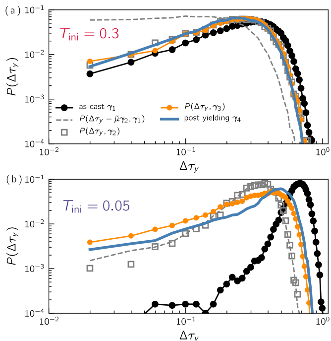
FIG. 9. Residual plastic strength distributions as a function of strain : Probability distribution of the residual plastic strength \Delta\tau_y at different strain corresponding to the state marked in Fig. 8(a) for a poorly annealed (a) and very stable glasses (b). Here P(\Delta\tau_y, \gamma_2) , P(\Delta\tau_y, \gamma_3) , and P(\Delta\tau_y, \gamma_4) is averaged over states at strain 4% < \gamma_2 < 5\% , 6% < \gamma_3 < 7\% , and \gamma_4 > 10\% , respectively.
