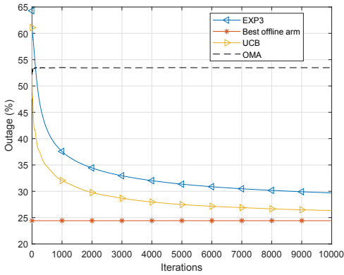
Fig. 1. Outage of adaptive NOMA (via UCB or EXP3) relying on a 1-bit feedback compared to OMA and the best offline policy. Our schemes greatly outperforms OMA in terms of outage probability.
