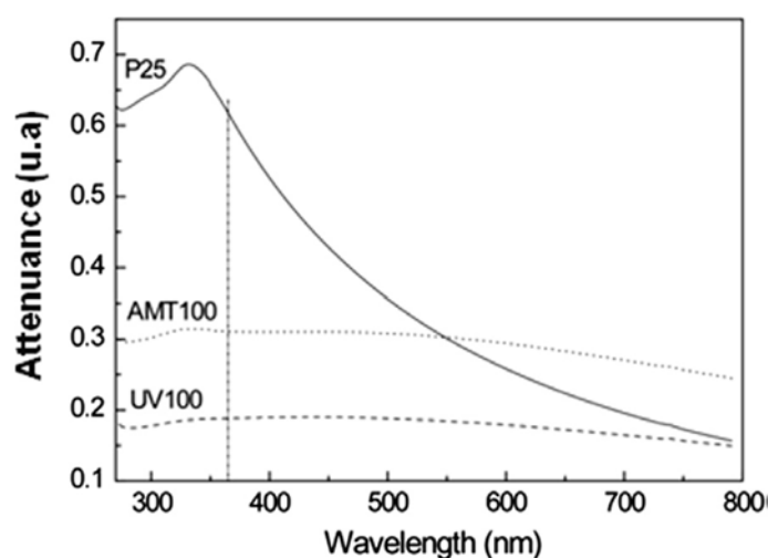
Fig. 1. UV-Vis attenuation spectra of nano-TiO 2 suspensions (0.025 g L -1 ) in 0.025 M EDTA (pH = 6.5): P25 (solid line), AMT100 (dotted line) and UV100 (dashed line). The vertical dotted line shows the excited wavelength ( \lambda = 365 nm) for the radical generation.
