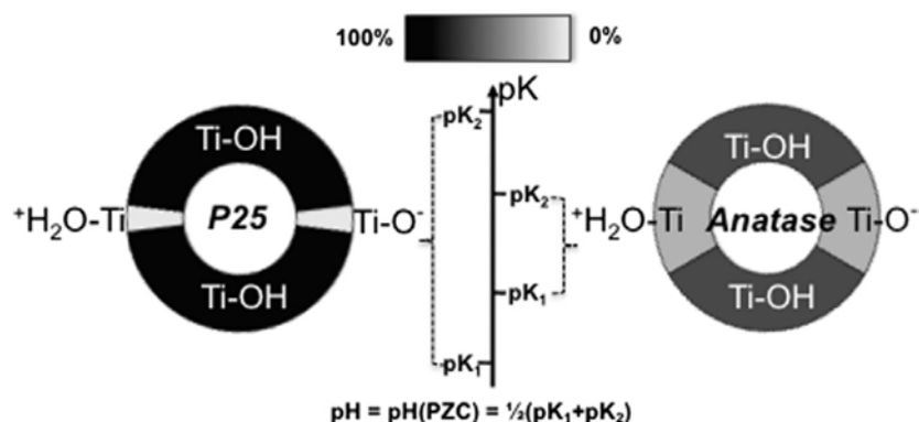
Scheme 3. Ideal relative proportion of the protonated–neutral-unprotonated surface groups, for pH = pH(PZC) , as a function of nano- TiO_2 origin: P25 (4–92–4% respectively) and Anatase (16.5–67–16.5% respectively).
