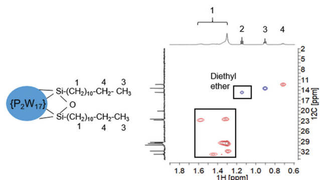
Fig. 3 C-H correlated NMR of POM-2C 12 illustrated by the POM-2C 12 molecular structure ({P 2 W 17 } represents {P 2 W 17 O 61 }), the square on the left of the 2D NMR graph labelled 1 is related to the 10 methylene groups labelled 1 in the POM-2C 12 molecular structure. Blue signals represent methyl groups and red for methylene groups.
