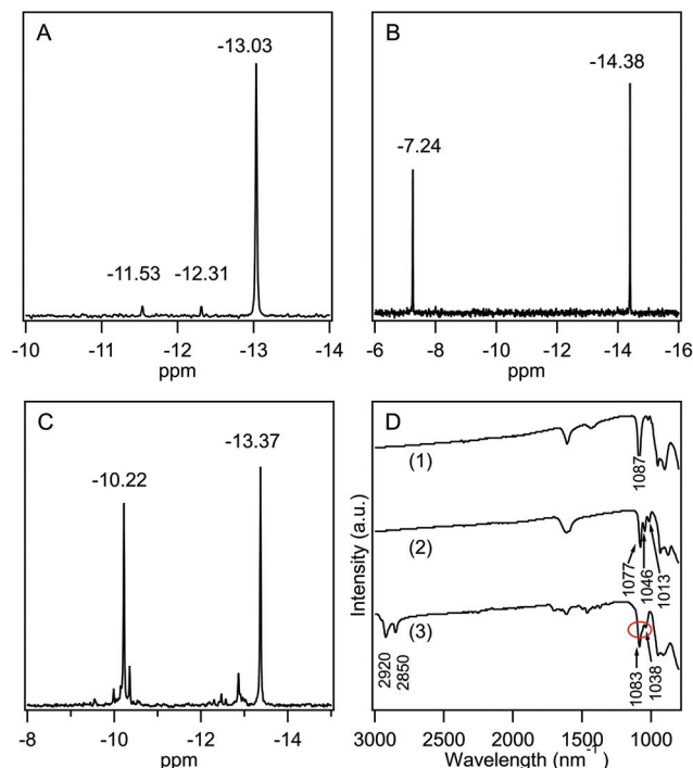
Fig. 2 31 P NMR spectra of (A) K 6 [α-P 2 W 18 O 62 ]·14H 2 O (B) K 10 [α 2 -P 2 W 17 O 61 ]·19H 2 O and (C) POM-2C 12 . (D) IR spectra of (1) K 6 [α-P 2 W 18 O 62 ]·14H 2 O (2) K 10 [α 2 -P 2 W 17 O 61 ]·19H 2 O and (3) POM-2C 12 (where the red circle indicates the existence of Dawson structured POM after tail grafting).
