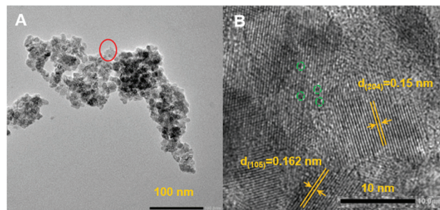
Fig. 9 (A) TEM and (B) HRTEM micrographs of the 12POM-TiO 2 material. HRTEM micrograph in (B) is a zoom of the region indicated with a red circle in (A). The dashed green circles in (B) are the possible locations of POMs in the 12POM-TiO 2 material.
