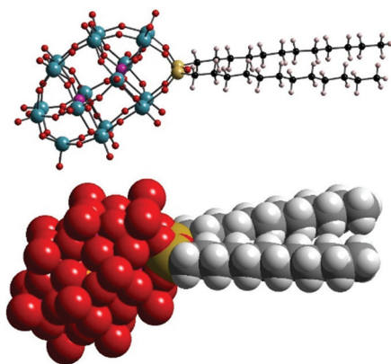
Fig. 1 Ball-and-stick and space-filling representations of the structure of the [P_2W_{17}O_{61}\{OSi_2(C_nH_{2n+1})_2\}]^{6-} anion ( R = C_{12}H_{25} ) POM-2C 12 . Colour code: W (blue), P (purple), O (red), Si (yellow), C (black) and H (white).
