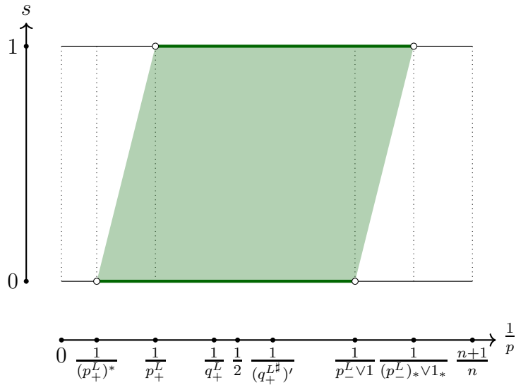
FIGURE 17. Exponents for uniqueness in Dirichlet and regularity problems in the case p_+(L) \leq n . Uniqueness holds on the open bottom and top segments (Sections 20.3 and 20.2) and the interior of the trapezoidal region (Section 20.6).
