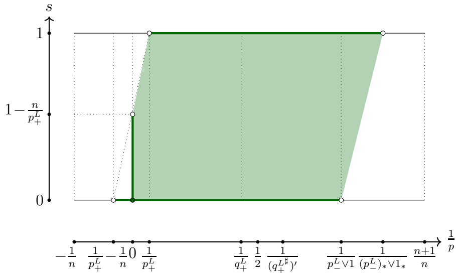
FIGURE 18. Exponents for uniqueness in Dirichlet and regularity problems in the case p_+(L) > n . Uniqueness holds on the open bottom and top segments (Sections 20.3, 20.2 and 20.5), the open vertical segment at 1/p = 0 and the interior of the trapezoidal region (Section 20.6). Exponents with 1/p < 0 correspond to the spaces \dot{\Lambda}^\alpha with \alpha = 1 - n/p as usual.
