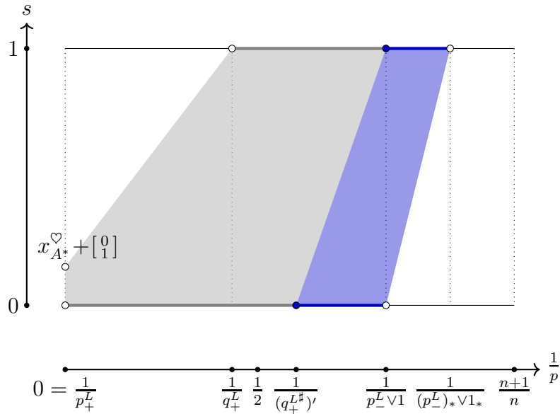
FIGURE 13. Extension of Figure 10 in the case p_-(L^\sharp) < 1 . This only concerns exponents with p \geq 2 . The length of the vertical segment on the left is at most n/p_-(L^\sharp) - n .
