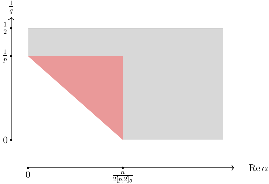
FIGURE 9. Visualization of the interpolation in Proposition 9.20. For (\operatorname{Re} \alpha, 1/q) in the interior of the grey shaded region, \mathbb{Q}_{\psi_\alpha, T} is bounded L^q \rightarrow T^q with a bound C e^{(\pi-2\mu)\operatorname{Im} \alpha} , where C is independent of \alpha . Stein interpolation in Step 3 provides boundedness L^q \rightarrow T^q in the interior of the red triangular region, the lower boundary of which is given by \frac{1}{q} = \frac{1}{p} - \frac{[p;2]_\theta}{p} \frac{2\operatorname{Re} \alpha}{n} .
