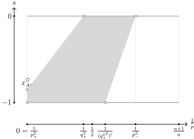
FIGURE 12. Extension of Figure 11 in the case p_-(L^\sharp) < 1 . The length of the vertical segment on the left is at most n/p_-(L^\sharp) - n .
