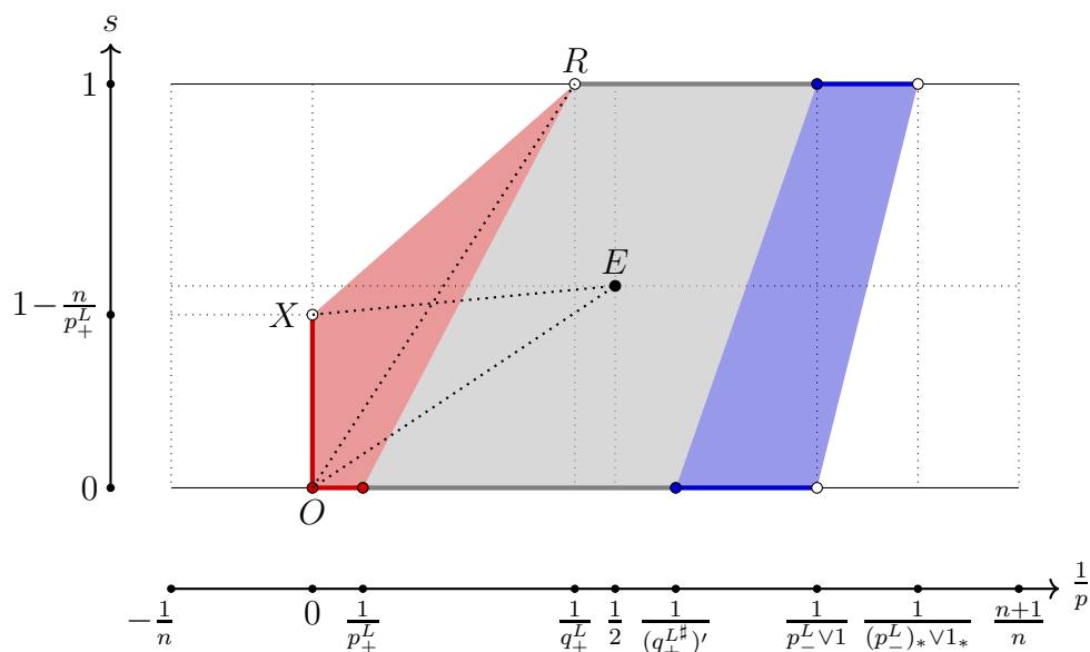
FIGURE 16. Extended region for compatible solvability if p_+(L) > n via a two-step interpolation argument. The picture is up to scale when p_+(L) < \infty but the coordinates of the colored regions' vertices are the same when p_+(L) = \infty . In this case X = (0, 1) . If even p_-(L^\sharp) < 1 , then parts of the red region also belongs to the extended gray identification region of Figure 13. This special situation has been showcased in Figure 3 in the introduction
