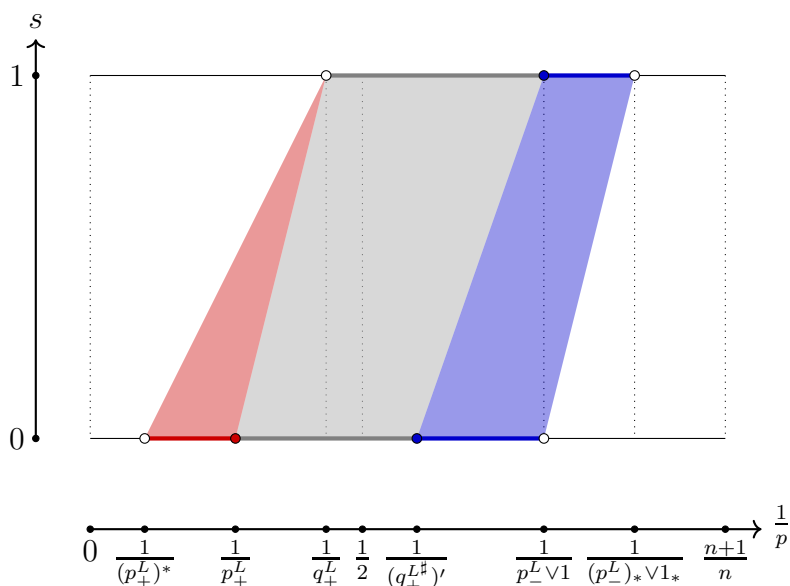
FIGURE 15. Extended region for compatible solvability of (D)_{X^{s,p}}^{\mathcal{L}} when p_+(L) < \infty . The figure is up to scale when p_+(L) < n but the coordinates of the colored trapezoid's vertices are the same when n \leq p_+(L) < \infty .
