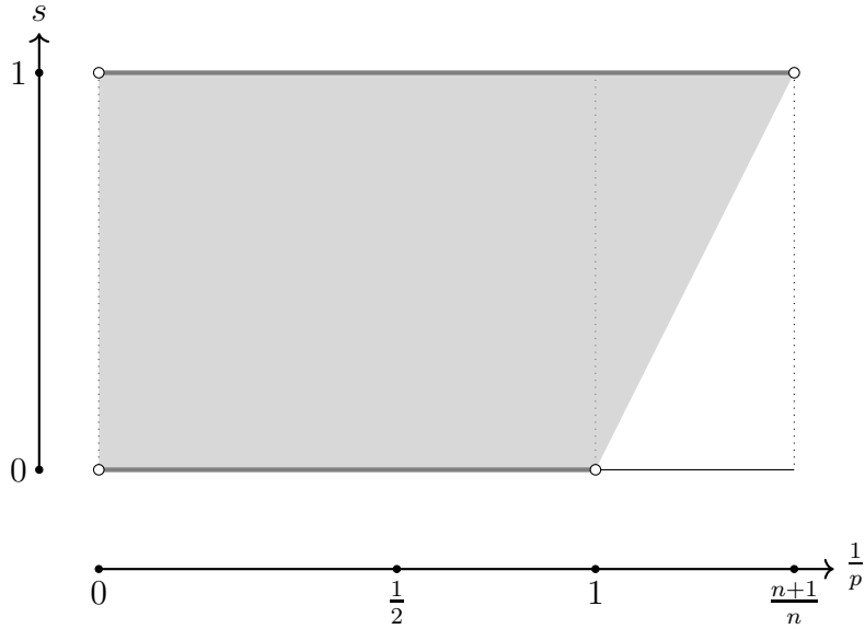
FIGURE 14. Figure 13 in dimension n = 1 or for the special case L = -a^{-1}\Delta_x in any dimension.
