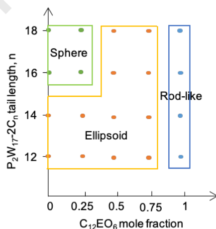
Figure 4. Phase diagram of binary P_2W_{17-2C_n}/C_{12}EO_6 mixtures at 8 and 16 mM, n , the carbon atom number in the hydrophobic P_2W_{17-2C_n} tails is given on the y-axis and the x-axis corresponds to the C_{12}EO_6 mole fraction.
