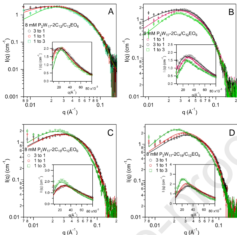
Figure 2. SANS data ( I(q) versus q ) and fits for h\text{-P}_2\text{W}_{17}\text{-}2\text{C}_n/h\text{-C}_{12}\text{EO}_6 with n= (A) 12 (B) 14 (C) 16 and (D) 18 at a total concentration of 8 mM in \text{D}_2\text{O} , given on a log-log scale. The insets correspond to the same scattering data plotted on a linear scale.
