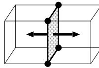
Fig. 8. An example of a case in which two adjacent unit cubes have a common 2-polyhedral candidate. If such 2-polyhedral candidates are extracted from \mathbf{V} , they are ignored for the construction of discrete closed surfaces.
