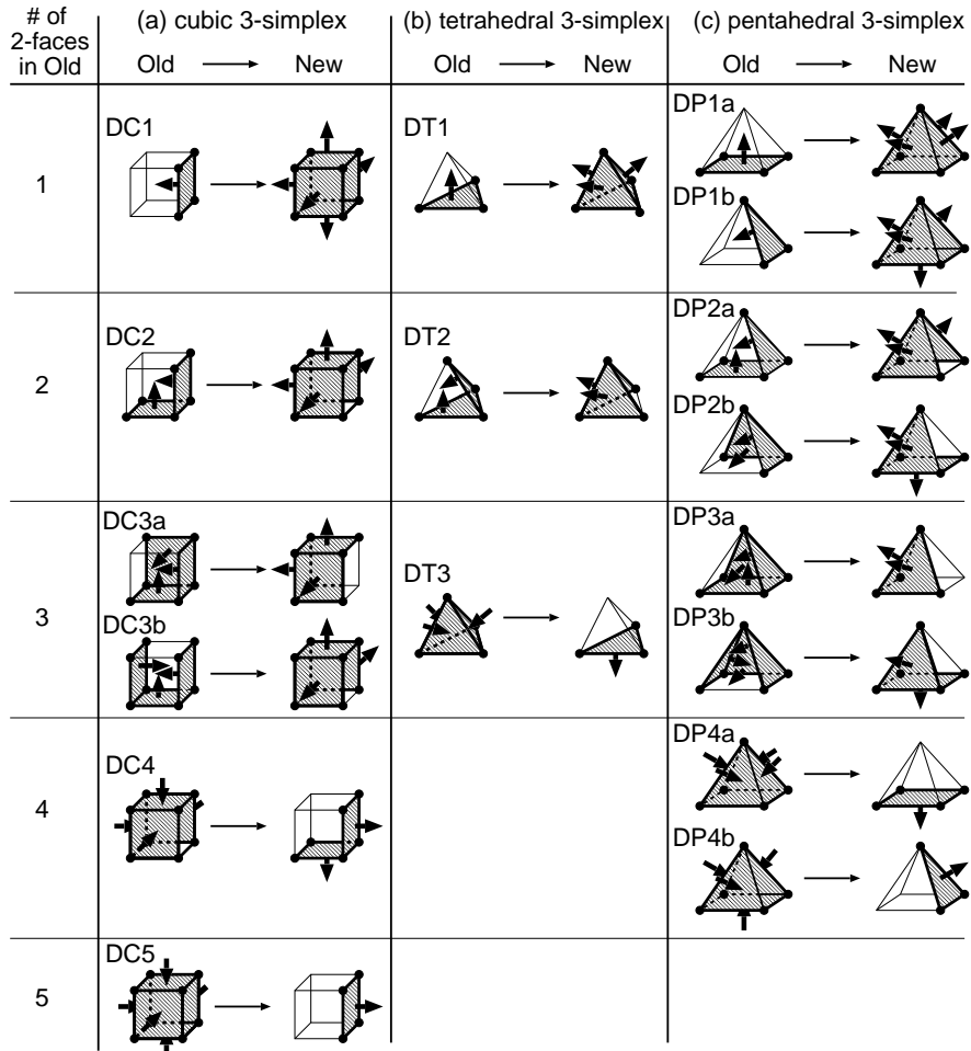
Fig. 11. All possible deformation operations for expanding \partial\mathbf{P} using a cubic 3-simplex in the 6-neighborhood system (a), using a tetrahedral 3-simplex in the 18- and 26-neighborhood systems (b), and using a pentahedral 3-simplex in the 18-neighborhood system (c). Note that \partial\mathbf{P} is expanded to (\partial\mathbf{P} \setminus \mathbf{Old}) \cup \mathbf{New} . Deformation operations for shrinking are obtained if we replace Old by New and New by Old respectively for each operation in this figure.
