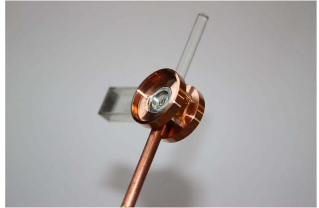
Figure 43. A complex gas target, manufactured by Scitech Precision, UK, for studying counterpropagating radiative shock collisions with X-ray radiography, generated from a petawatt laser beam, as a primary diagnostic used on experiments on SG-II at SIOM, China (picture courtesy of Imperial College London).
