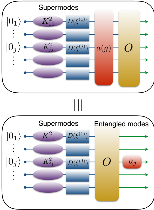
FIG. 1. Circuit representation of Eqs. (78)–(80) for a pure initial state \rho_G , represented in the mode basis obtained by the Bloch-Messiah decomposition (blue lines) as a vacuum (|0_1\rangle \otimes \dots \otimes |0_m\rangle) that is locally squeezed K_{jj}^2 and displaced D(\xi^{(j)}) . The top panel shows that general photon subtraction is implemented by the action of annihilation a(g) in mode g \in \mathcal{N}(\mathbb{R}^{2m}) , which is nonlocal (see the text) in the supermode basis. The mode basis is changed by the action of a linear optics operation (78), characterized by an orthogonal symplectic matrix O . The bottom panel shows the equivalent procedure (80), where the mode basis is changed (green lines) before subtracting the photon. Here we assume that O'g = e^{(j)} , which is one of the modes in the new mode basis (green lines) such that the subtraction is local. We define a_j = a(e^{(j)}) .
