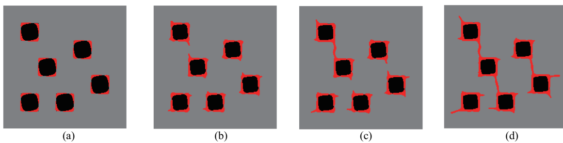
Figure 17. Crack propagation in the initial composite with randomly distributed inclusions subjected to loading case 3: (a) \bar{U} = 5 mm; (b) \bar{U} = 10 mm; (c) \bar{U} = 11 mm; (d) \bar{U} = 12 mm.
