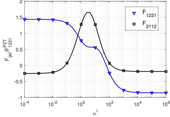
Fig. 9. Evolution of effective flexoelectric components with respect to dielectric properties the inclusion for the RVE with triangular inclusions.
