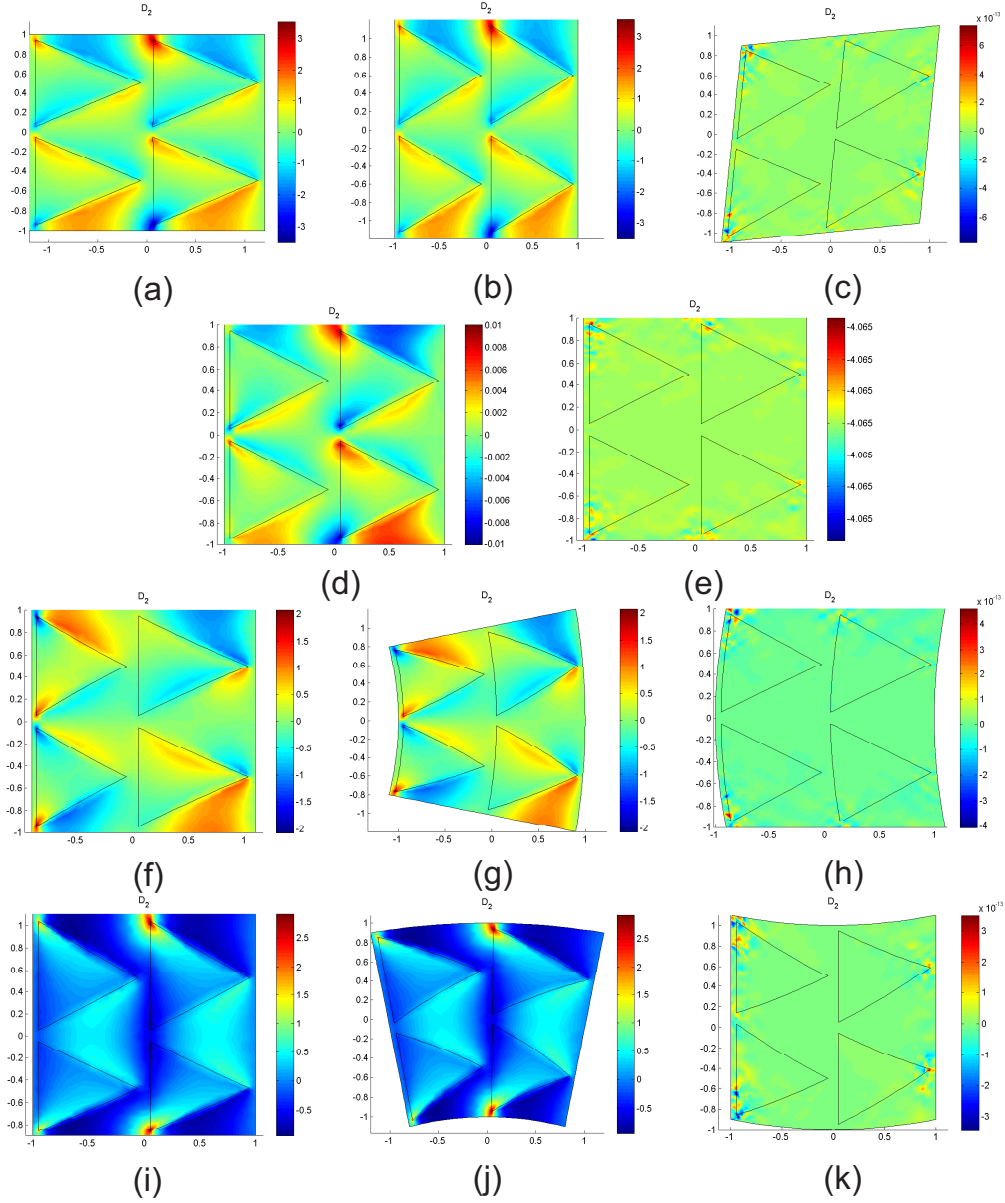
Fig. 3. d_2(\mathbf{x}) electric displacement field in deformed ( \times 0.2 ) configurations for RVE with triangular inclusions: (a) [\bar{\boldsymbol{\varepsilon}}] = [1; 0; 0] , \bar{\nabla}\boldsymbol{\varepsilon} = \mathbf{0} , \bar{\mathbf{E}} = \mathbf{0} ; (b) [\bar{\boldsymbol{\varepsilon}}] = [0; 1; 0] , \bar{\nabla}\boldsymbol{\varepsilon} = \mathbf{0} , \bar{\mathbf{E}} = \mathbf{0} ; (c) [\bar{\boldsymbol{\varepsilon}}] = [0; 0; 1/2] , \bar{\nabla}\boldsymbol{\varepsilon} = \mathbf{0} , \bar{\mathbf{E}} = \mathbf{0} ; (d) [\bar{\boldsymbol{\varepsilon}}] = \mathbf{0} , \bar{\nabla}\boldsymbol{\varepsilon} = \mathbf{0} , [\bar{\mathbf{E}}] = [1; 0] ; (e) [\bar{\boldsymbol{\varepsilon}}] = \mathbf{0} , \bar{\nabla}\boldsymbol{\varepsilon} = \mathbf{0} , [\bar{\mathbf{E}}] = [0; 1] ; (f) [\bar{\boldsymbol{\varepsilon}}] = \mathbf{0} , \bar{\nabla}\boldsymbol{\varepsilon} = [1; 0; 0; 0; 0; 0] , \bar{\mathbf{E}} = \mathbf{0} ; (g) [\bar{\boldsymbol{\varepsilon}}] = \mathbf{0} , \bar{\nabla}\boldsymbol{\varepsilon} = [0; 1; 0; 0; 0; 0] , \bar{\mathbf{E}} = \mathbf{0} ; (h) [\bar{\boldsymbol{\varepsilon}}] = \mathbf{0} , \bar{\nabla}\boldsymbol{\varepsilon} = [0; 0; 1; 0; 0; 0] , \bar{\mathbf{E}} = \mathbf{0} ; (i) [\bar{\boldsymbol{\varepsilon}}] = \mathbf{0} , \bar{\nabla}\boldsymbol{\varepsilon} = [0; 0; 0; 1; 0; 0] , \bar{\mathbf{E}} = \mathbf{0} ; (j) [\bar{\boldsymbol{\varepsilon}}] = \mathbf{0} , \bar{\nabla}\boldsymbol{\varepsilon} = [0; 0; 0; 0; 1; 0] , \bar{\mathbf{E}} = \mathbf{0} ; (k) [\bar{\boldsymbol{\varepsilon}}] = \mathbf{0} , \bar{\nabla}\boldsymbol{\varepsilon} = [0; 0; 0; 0; 0; 1] , \bar{\mathbf{E}} = \mathbf{0} .
