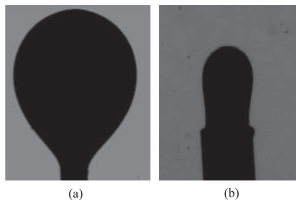
Fig. 5. Images of pendant drop for measurement of IFT between the oil and aqueous solutions, (a) \text{MgSO}_4 solution at 50 000 ppm, (b) \text{Na}_2\text{CO}_3 solution at 60 000 ppm.
