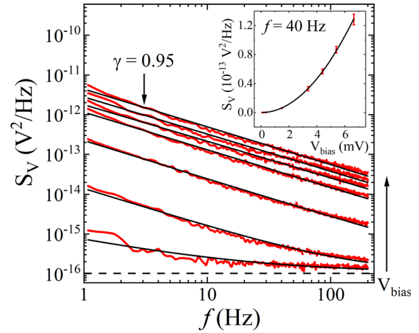
FIG. 2. Bias dependence of the low-frequency noise of sample #1 (red lines) measured at 77 K. The applied bias voltages are V_{bias} = 0.085, 0.33, 1.48, 3.37, 4.40, 5.39, and 6.65 mV, respectively. At low bias, the S_V vs f curve is just above the estimated Johnson-Nyquist level (dashed line, calculated using the measured resistance R(77\text{ K}) = 23.5 k \Omega ). At high bias, curves are dominated by a 1/f^\gamma dependence, with the value of \gamma consistently between 0.9 and 1.1. Black lines are best fits to the data using Eq. (1). Specifically, when V_{bias} = 6.65 mV, \gamma = 0.95 . (Inset) S_V taken at 40 Hz as a function of V_{bias} . The black line is the best fit to the data using Eq. (1) with f = 40 Hz and \gamma = 1 .
