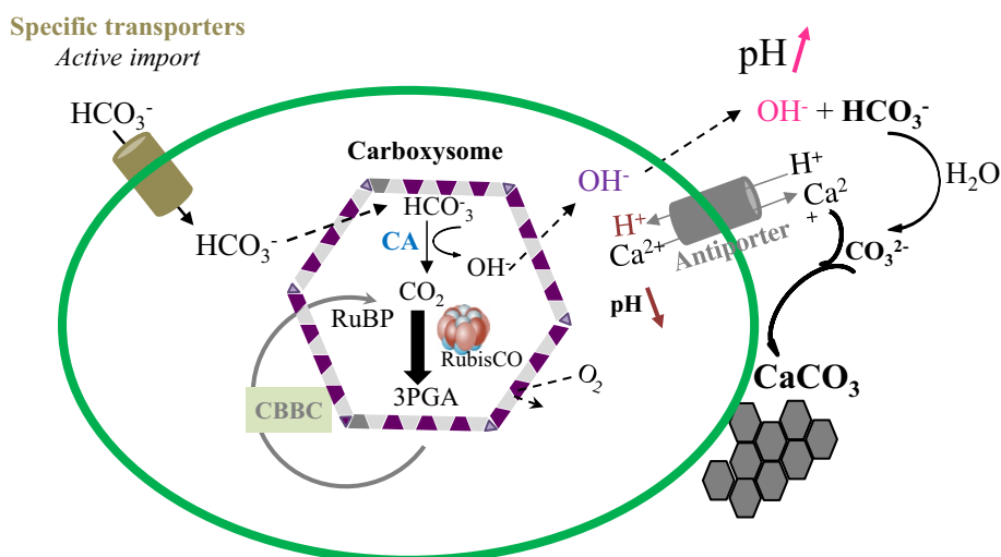
Fig. 3 Simplified model of CCM-dependent biologically induced mineralization of \text{CaCO}_3 . Carbon concentrating mechanism CCM involves the uptake of \text{HCO}_3^- . Carbonic anhydrase (CA) converts \text{CO}_2 into \text{HCO}_3^- in the cytoplasm and \text{HCO}_3^- into \text{CO}_2 in the carboxysome. \text{CO}_2 is fixed by RubisCO and used by the Calvin-Benson-Bassham Cycle (CBBC). Conversion of \text{HCO}_3^- into \text{CO}_2 releases \text{OH}^- . To buffer intracellular pH, specific transporters such as \text{Ca}^{2+}/\text{H}^+ antiporters import \text{H}^+ and export \text{Ca}^{2+} . The import of \text{H}^+ inside the cell lead to an increase of the extracellular pH, which together with export of \text{Ca}^{2+} favors the precipitation of extracellular \text{CaCO}_3 [20, 30, 172]
