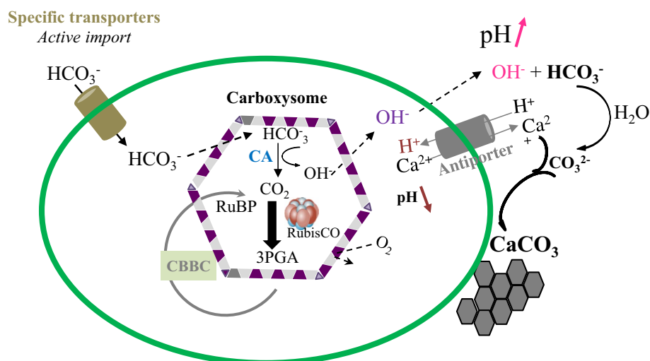
Fig. 3 Simplified model of CCM-dependent biological induced mineralization of \text{CaCO}_3 . Carbon concentrating mechanism CCM involves the uptake of \text{HCO}_3^- . Carbonic anhydrase (CA) converts \text{CO}_2 into \text{HCO}_3^- in the cytoplasm and \text{HCO}_3^- into \text{CO}_2 in the carboxysome. \text{CO}_2 is fixed by RubisCO and used by the Calvin-Benson-Bassham Cycle (CBBC). Conversion of \text{HCO}_3^- into \text{CO}_2 releases \text{OH}^- . To buffer intracellular pH, specific transporters such as \text{Ca}^{2+}/\text{H}^+ antiporters import \text{H}^+ and export \text{Ca}^{2+} . The import of \text{H}^+ inside the cell lead to an increase of the extracellular pH, which together with export of \text{Ca}^{2+} favors the precipitation of extracellular \text{CaCO}_3 [20, 30, 172]
