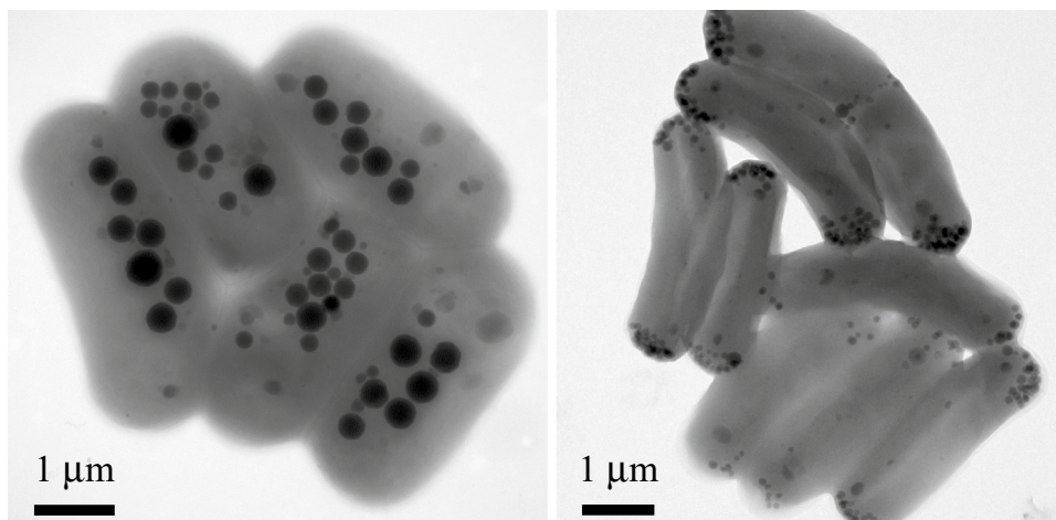
Fig. 5 Transmission electron microscopy images in the bright field mode of ACC-forming cyanobacteria: a Cyanothecce sp. PCC 7425 cells showing ACC inclusions (darkest inclusion) scattered throughout the cells; b Synechococcus lividus PCC 6716 cells showing ACC inclusions (darkest inclusions) located at the septum and the poles of the cells [43]. Some brighter inclusions are also visible in both strains and correspond to polyphosphate granules. Identification of polyphosphate and ACC granules was achieved by Benzerara et al. [43] based on STEM-EDX mapping, electron diffraction and XANES spectroscopy at the C K-edge and Ca L_{2,3} -edges
