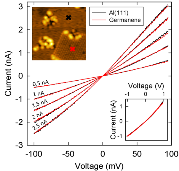
FIG. 5. I-V curve measured as a function of setpoint current on Al(111) and germanene areas indicated by crosses in the STM image of the upper inset at 5 K. Inset: similar I(V) curves measured on a wider bias range with a setpoint current of 1 nA.
