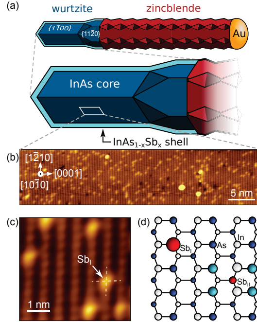
Figure 1: (a) Schematic of the [\bar{1}\bar{1}\bar{1}] grown WZ structure InAs core in blue and the axially grown \text{InAs}_{1-x}\text{Sb}_x ZB structure in red. During axial growth an additional lateral overgrowth on the sidewall facets of the InAs core by WZ structure \text{InAs}_{1-x}\text{Sb}_x occurs (light blue). (b) Atomically resolved constant-current STM image of the overgrown sidewall surface measured at 77 K, using a sample voltage of -3 V and a tunnel current of 10 pA. Under these tunneling conditions, the filled dangling bond states above the surface anions are imaged. (c) Magnified STM image showing the atomic rows in detail. The bright atomically localized contrast features arise from substitutional Sb atoms on As sites. (d) Atomic ball model of Sb atoms in different subsurface layers (same orientation as the STM image), illustrating different symmetries of the Sb contrast on the surface: Sb atoms incorporated on As sites in the surface layer (denoted as \text{Sb}_I ) can be observed as protrusions centered on top of an anion sublattice site in the STM image. In contrast, Sb atoms incorporated in the second atomic layer ( \text{Sb}_{II} ) can be anticipated to give rise to an outward relaxation of four surface As atoms (light blue balls) and thus a protrusion centered inbetween of the atomic chains. Since such contrast features are never observed, the second atomic layer is free of Sb, indicating the presence of only a single monolayer thick \text{InAs}_{1-x}\text{Sb}_x shell.
