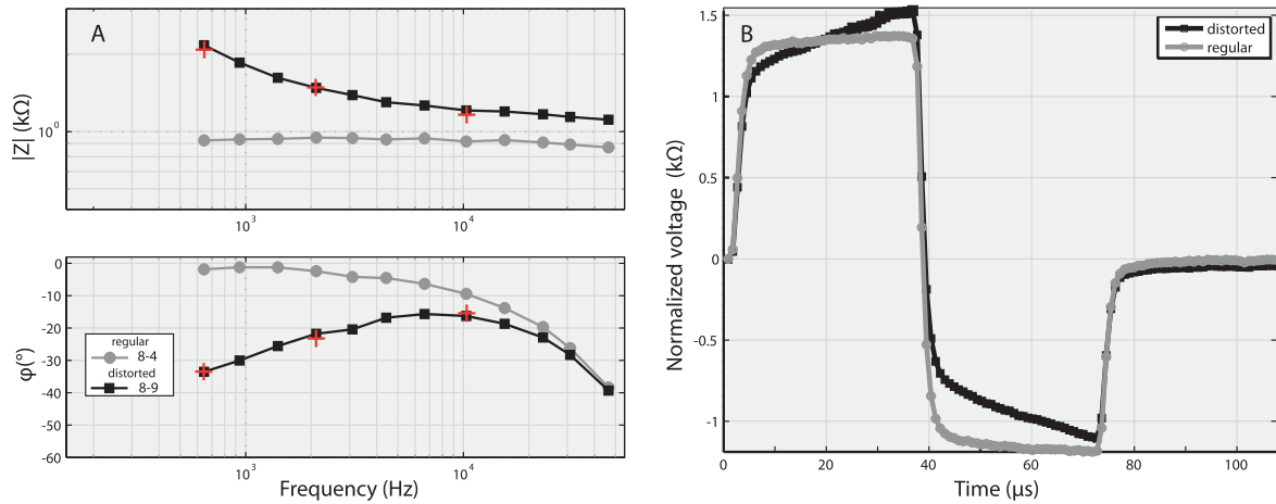
Figure 4. Panel (A) Bode diagram from transimpedance spectroscopy with 10 \mu A stimuli measured in S5. Regular data (grey circles) were recorded using stimulating-recording electrodes 8–4 and distorted data (black squares) were recording using electrodes 8–9. Red + symbols represent additional data recorded using electrodes 8–9, with an amplitude of 5 \mu A . Panel (B) Up-sampled transimpedance waveforms for 50 \mu A biphasic pulse input measured in S5. Regular data (grey circles) were recorded using stimulating-recording electrodes 1–2 and distorted data (black squares) were recording using electrodes 8–9.
