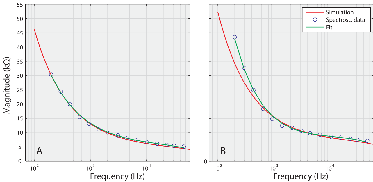
Figure 14. Examples of magnitude spectra of contact impedance for subject S7, panel A and subject S1, panel (B). The circles indicate the spectroscopy data points, the green curves represent the output of the contact impedance model applied on the spectroscopy data and the red curves represent the simulated spectrum based on the model estimations obtained using biphasic pulses.
