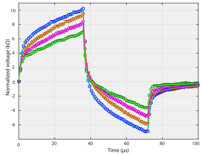
Figure 9. Four examples of contact impedance waveforms (each symbol is for one electrode) and model output (Solid lines) measured with S2 in the default condition ( 50 \mu\text{A} biphasic pulses with a 35.92 \mu\text{s} phase duration).
