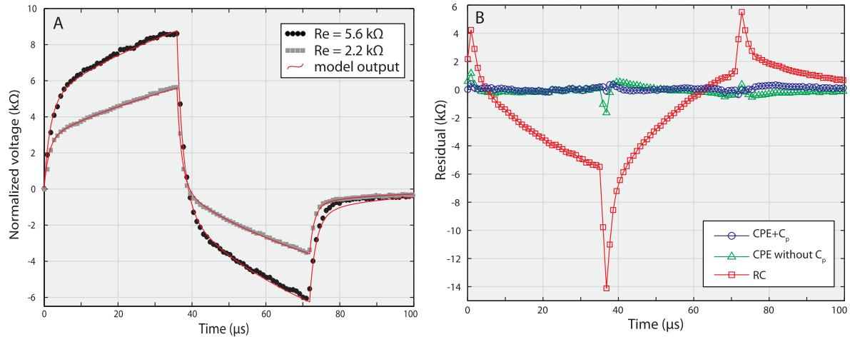
Figure 8. Panel (A) Contact impedance waveforms recorded in vitro for R_e = 2.2 \text{ k}\Omega (grey squares) and 5.6 \text{ k}\Omega (black dots) and model outputs. Panel (B) Residual of different contact impedance model fittings: a resistor-capacitor (RC) model similar to what is commonly used to fit CI impedance data ((Newbold et al 2004, Vanpoucke et al 2004a, Tykocinski et al 2005), squares), the model with a CPE presented in figure 7 with (circles) and without C_p (triangles).
