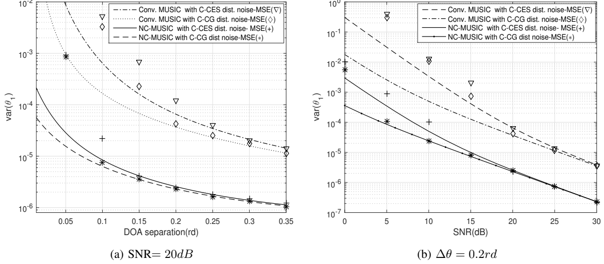
Fig. 1. Asymptotic variances \text{var}(\theta_{1,T}) given by (37)-(38) and (39)-(40) and its associated MSEs versus SNR (and versus DOA separation \Delta\theta = |\theta_2 - \theta_1| ) for C-CG and circular complex Student t -distributed noise models with \nu = 4.1 , fixed DOAs and phases with \Delta\phi \stackrel{\text{def}}{=} |\phi_2 - \phi_1| = 0.1rd and \rho = |\rho'| = 0.5 .
