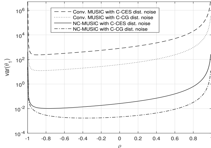
Fig. 3. Asymptotic variances \text{var}(\theta_{1,T}) associated with conventional MUSIC [resp., NC MUSIC] algorithm given by (40) [resp., by (38)] for C-CG noise model, and by (39) [resp., (37)] for circular complex Student t -distributed noise model with \nu = 4.1 and \text{SNR} = 20\text{dB} .
