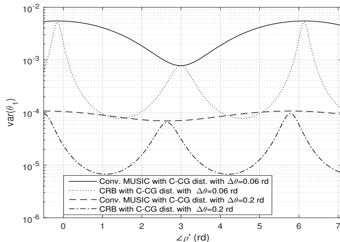
Fig. 4. Asymptotic variance \text{var}(\theta_{1,T}) associated with the conventional MUSIC algorithm given by (40) for C-CG distributed observations, compared to the stochastic CRB, for different values of \Delta\theta with |\rho'| = 0.95 , \text{SNR} = 20\text{dB} and T = 2000 .
