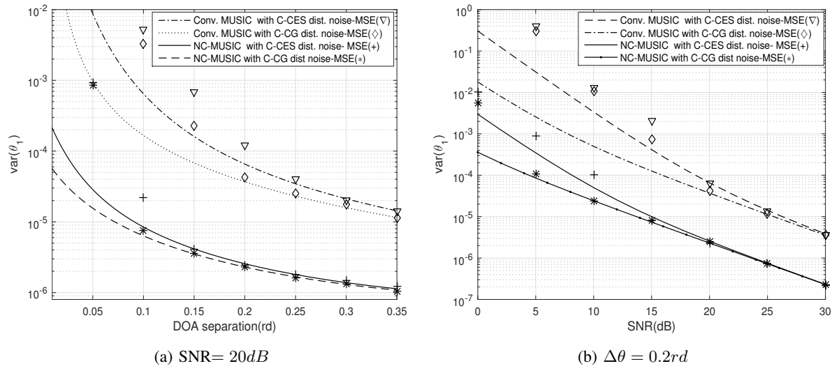
Fig. 1. Asymptotic variances \text{var}(\theta_{1,T}) given by (37)-(38) and (39)-(40) and its associated MSEs versus SNR (and versus DOA separation \Delta\theta = |\theta_2 - \theta_1| ) for C-CG and circular complex Student t -distributed noise models with \nu = 4.1 , fixed DOAs and phases with \Delta\phi \stackrel{\text{def}}{=} |\phi_2 - \phi_1| = 0.1rd and \rho = |\rho'| = 0.5 .
