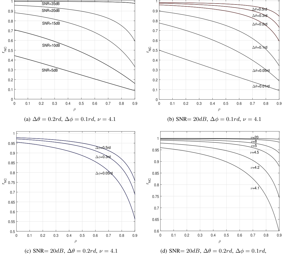
Fig. 2. Ratio between (37) and (38) (denoted by r_{NC} \stackrel{\text{def}}{=} R_G^{NC}(\theta_1)/R_{NG}^{NC}(\theta_1) ) as a function of \rho for different values of SNR, \Delta\theta , \Delta\phi and \nu .
