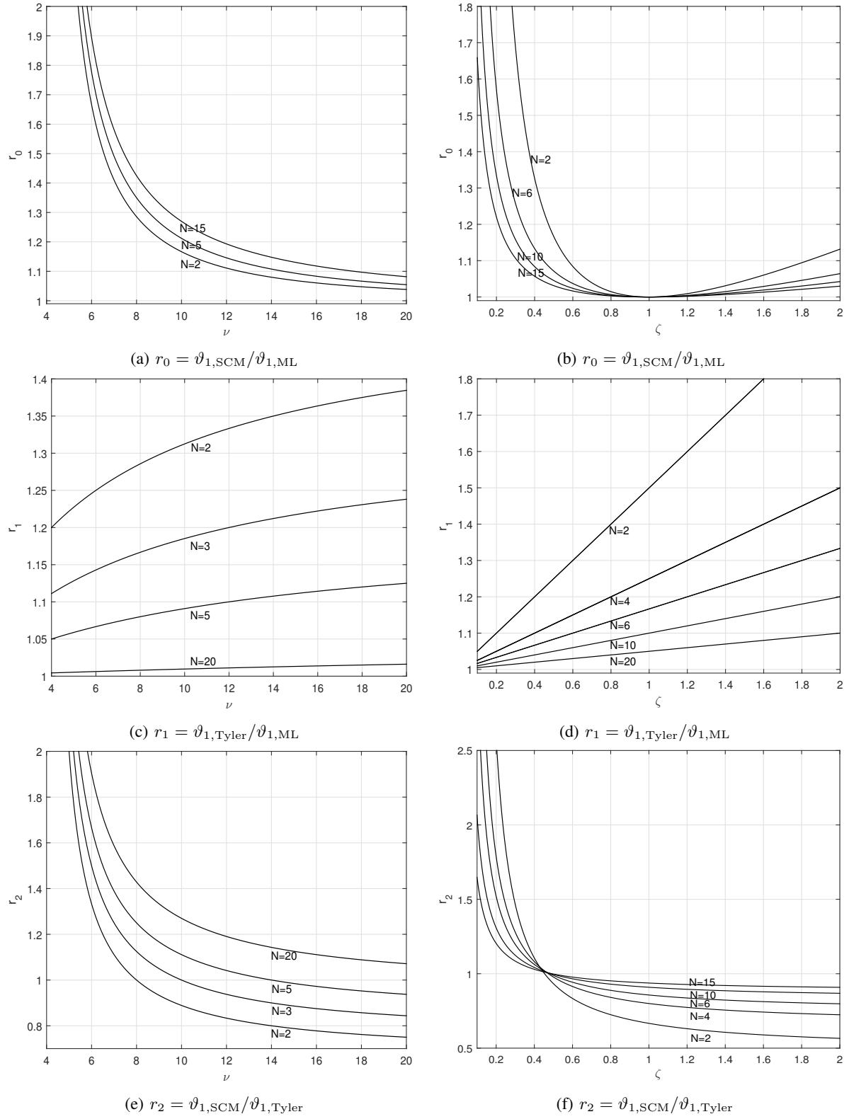
Fig. 5. Ratios r_0 = \vartheta_{1,\text{SCM}}/\vartheta_{1,\text{ML}} , r_1 = \vartheta_{1,\text{Tyler}}/\vartheta_{1,\text{ML}} and r_2 = \vartheta_{1,\text{SCM}}/\vartheta_{1,\text{Tyler}} versus NC complex Student t -distribution parameter \nu (first column) and versus NC complex generalized Gaussian distribution parameter \zeta (second column) for different values of N .
