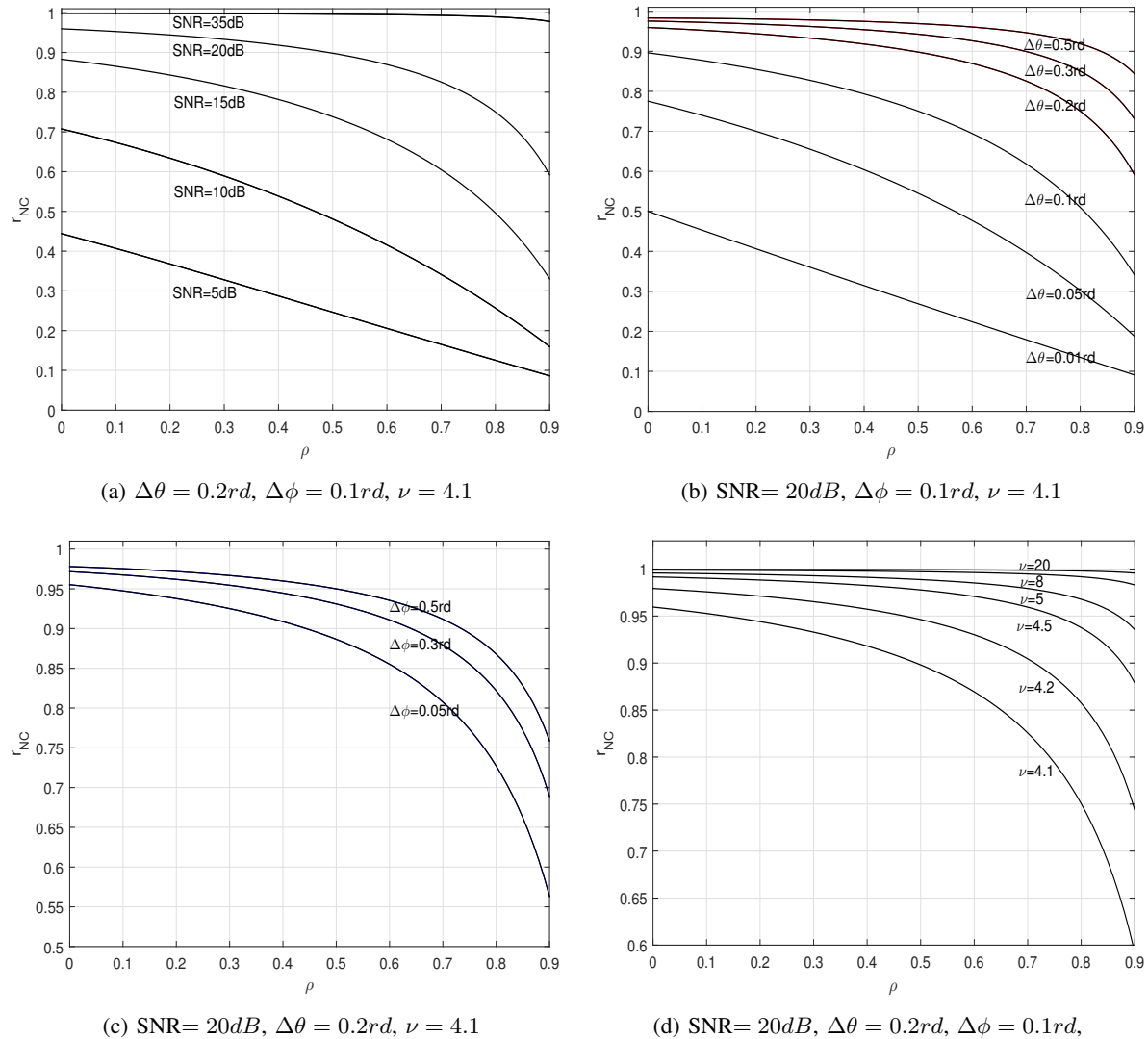
Fig. 2. Ratio between (37) and (38) (denoted by r_{\text{NC}} \stackrel{\text{def}}{=} R_{\text{G}}^{\text{NC}}(\theta_1)/R_{\text{NG}}^{\text{NC}}(\theta_1) ) as a function of \rho for different values of SNR, \Delta\theta , \Delta\phi and \nu .
