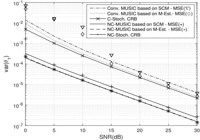
Fig. 6. Circular and NC stochastic CRBs, asymptotic variances given by (29) and [26, Eq.(34)] and associated MSEs versus SNR for NC complex generalized Gaussian distributed observations with exponent \zeta = 0.2 , fixed DOAs and phases with \Delta\theta = 0.25(rd) and \Delta\phi = 0.2(rd) , and \rho = |\rho'| = 0.5 .
