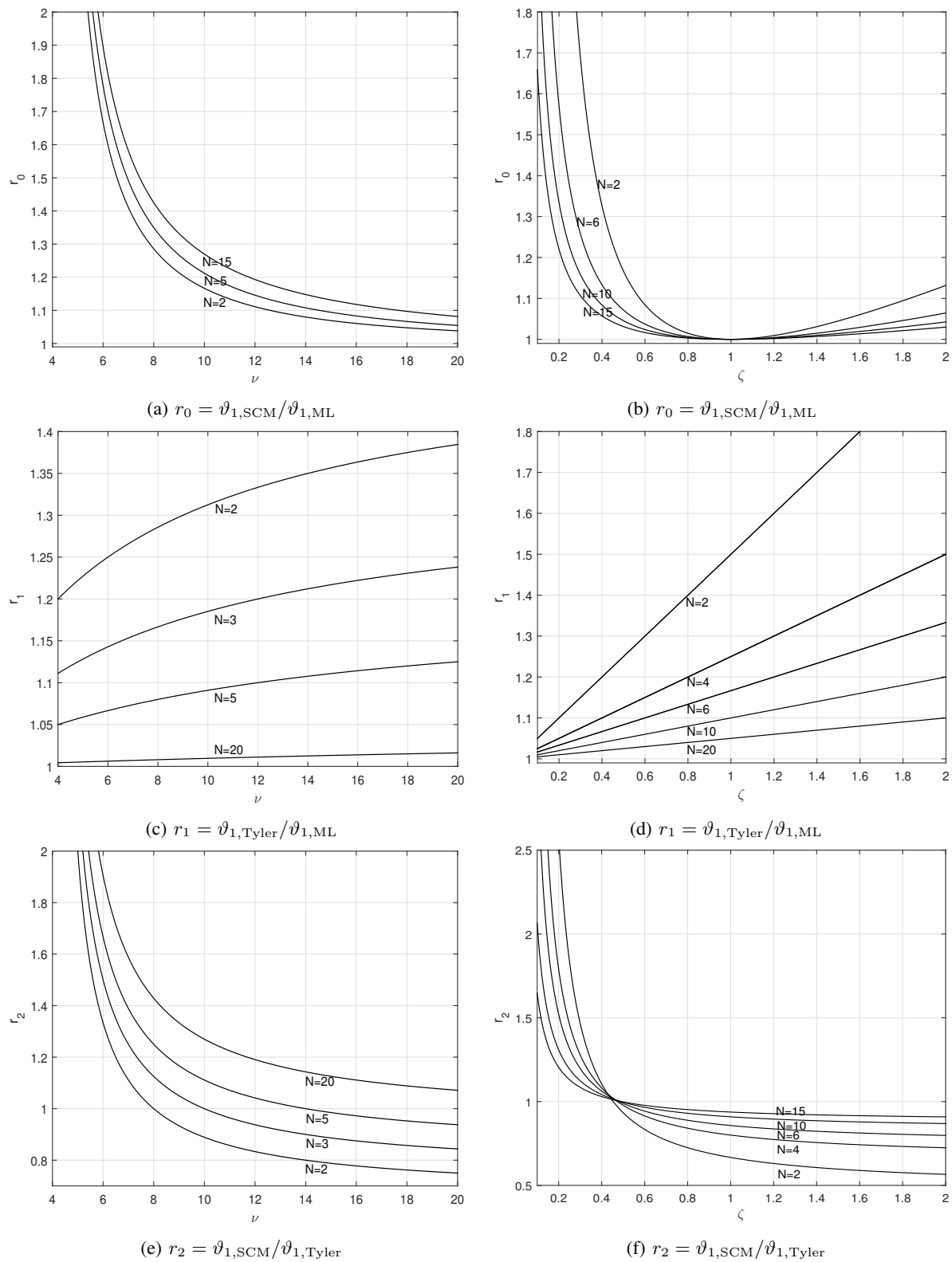
Fig. 5. Ratios r_0 = \vartheta_{1,SCM}/\vartheta_{1,ML} , r_1 = \vartheta_{1,Tyler}/\vartheta_{1,ML} and r_2 = \vartheta_{1,SCM}/\vartheta_{1,Tyler} versus NC complex Student t -distribution parameter \nu (first column) and versus NC complex generalized Gaussian distribution parameter \zeta (second column) for different values of N .
