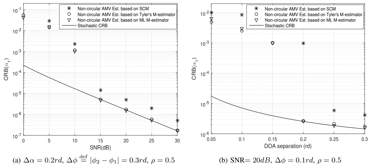
Fig. 1. Non-circular stochastic CRB (45) and MSEs obtained with AMV subspace-based estimator (18) build from \mathbf{\Pi}_{\tilde{y},K} versus SNR (and versus DOA separation \Delta\alpha = |\alpha_2 - \alpha_1| ) for non-circular complex Student t -distributed observations with \nu = 4.1 .
