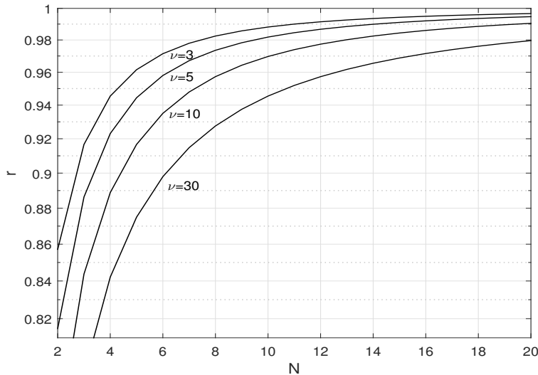
Fig.2. Ratio r \stackrel{\text{def}}{=} R_{\alpha_1, \text{ML}}^{\text{AMV(II)}} / R_{\alpha_1, \text{Tyler}}^{\text{AMV(II)}} versus N for different values of \nu .
