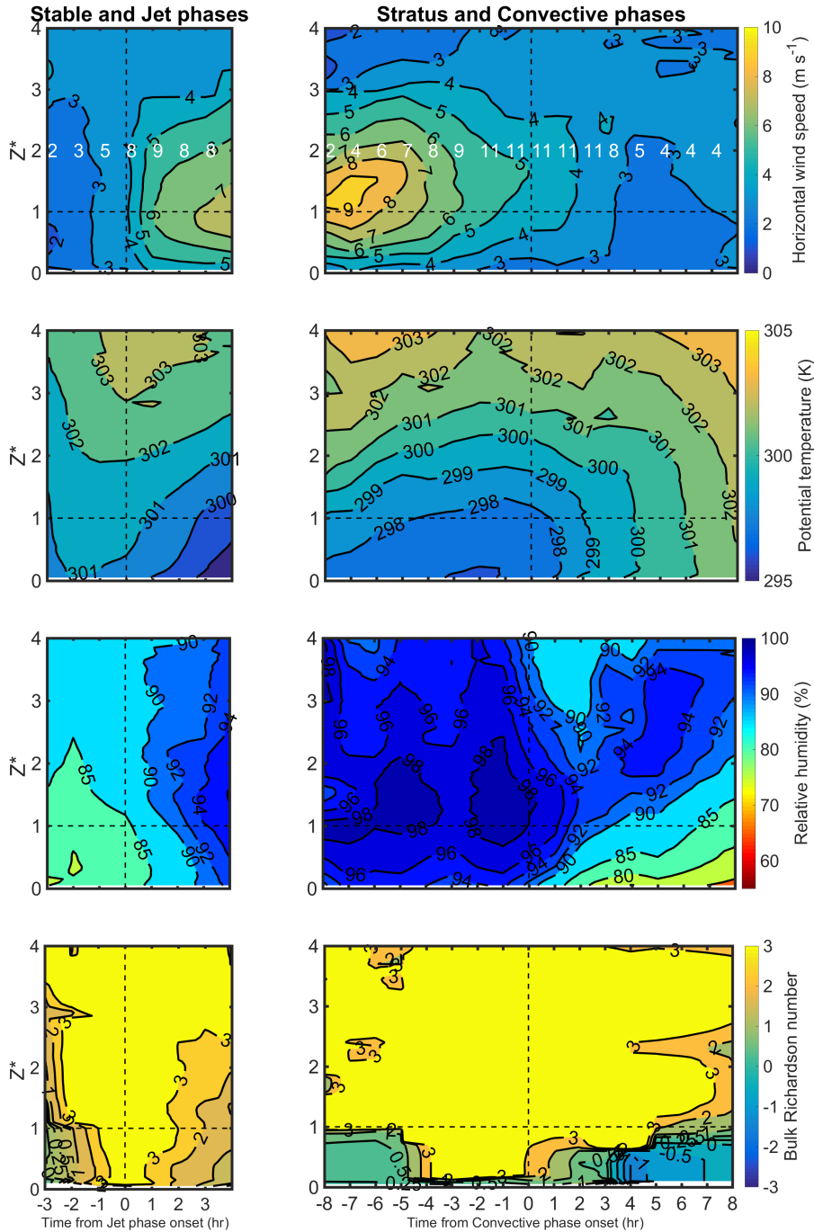
Figure 3. Mean height-time sections for, from top to bottom, horizontal wind speed ( \text{m s}^{-1} ), potential temperature (K), relative humidity (%) and Bulk Richardson number (colour scale and isolines). These height-time sections are built by (i) normalising the height by the CBH when the stratus clouds form for each individual radiosounding, (ii) setting the origin of time with a time reference appropriately chosen according to the considered phase, and (iii) hourly averaging the radiosoundings. The origin of time is set to (left column) MI arrival time (negative and positive times standing for stable and jet phases, respectively), and (right column) start of the convective phase ( H > 10 \text{ W m}^{-2} ) (negative and positive times standing for stratus phase and convective phase, respectively). The horizontal dashed line ( Z_* = 1 ) indicates the CBH when the stratus clouds form. White numbers in the top panels indicate the number of radio soundings available for the hourly-average.
