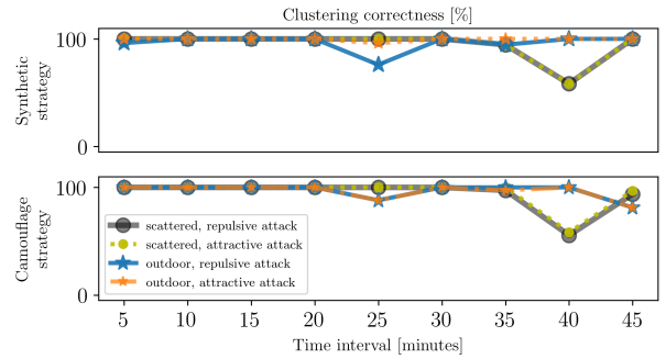
Fig. 8. Percentage of clustering correctness for online detection.
