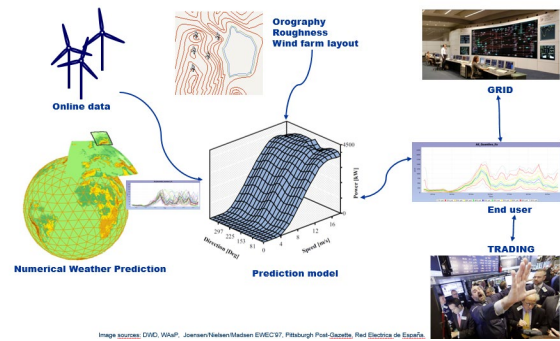
Figure 1: The general data flow in a short-term forecasting model.
