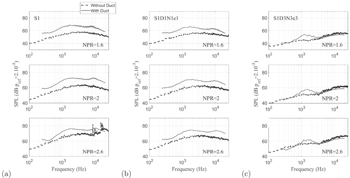
Fig. 14. Comparison of the mixing noise with and without duct at \theta = 90^\circ for: (a) diaphragm S1, (b) perforated plates S1D1N1e1 and (c) S1D3N3e3.
