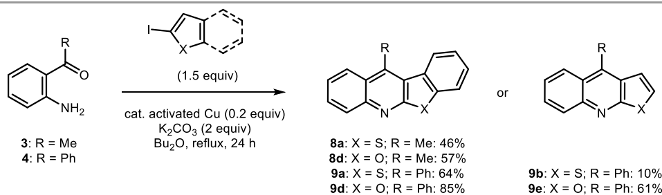
Scheme 1 Results obtained in the frame of a previous study. 17b
