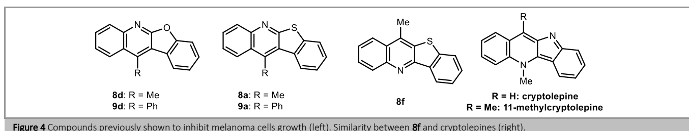
Figure 4 Compounds previously shown to inhibit melanoma cells growth (left). Similarity between 8f and cryptolepines (right).
