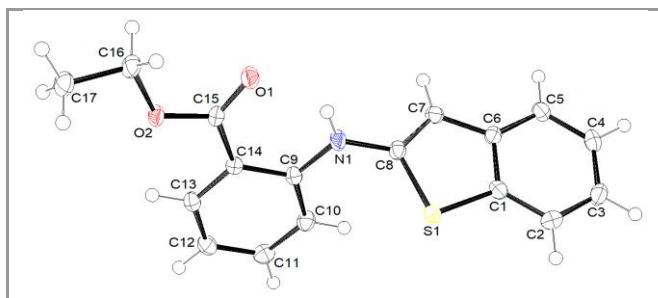
Figure 1 ORTEP diagram (50% probability) of the compound 2b .
