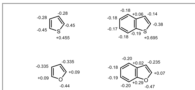
Figure 2 Mulliken charges on atoms calculated (MP2/6-31G(d)) by Belen'kii, Suslov and Chuvytkin for thiophene, benzo[ b ]thiophene, benzo[ b ]furan and furan. 24
