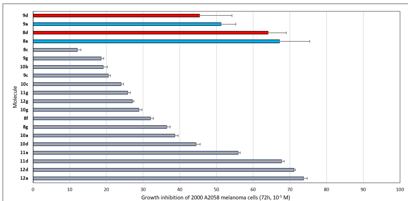
Figure 5 Antiproliferative activity of four compounds previously evaluated (top, colored) and of 16 of the compounds here synthesized (bottom, grey) at 10 -5 M after 72 h in A2058 human melanoma cells.
