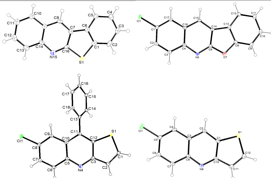
Figure 3 ORTEP diagrams (50% probability) of the compounds 10a , 12d , 11g and 12g .
