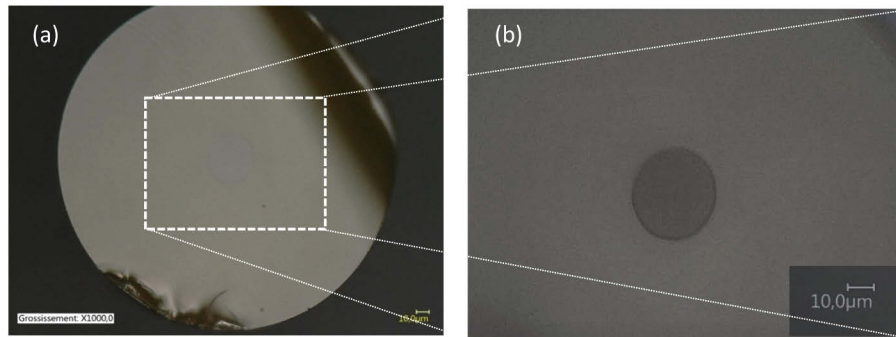
Fig. 8. (a) Microscope image of the cross section of the fibre. The total and the core diameters were measured at 300 µm and 35 µm, respectively; (b) Microscope image zoom on the core/clad interface.
