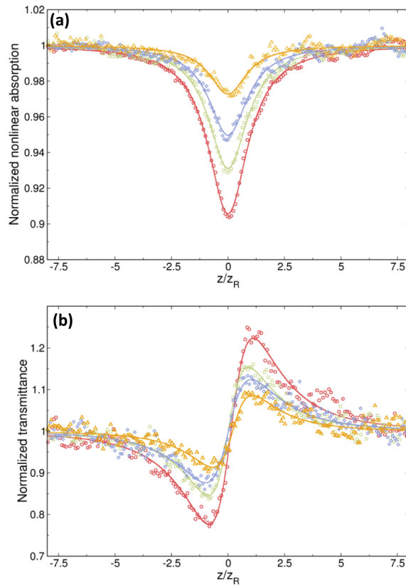
Fig. 1. Typical plots of the nonlinear absorption \beta (a) and normalized transmittance (b) for different values of the irradiance for glass samples. The data were recorded for the specific composition ([\text{GeS}_2]_{0.80}[\text{Ga}_2\text{S}_3]_{0.20})_{95}(\text{CsCl})_5 .
