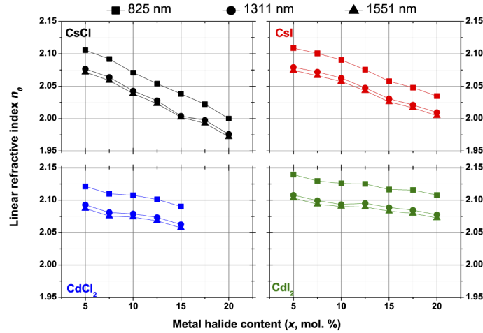
Fig. 6. Evolution of the linear refractive index of glasses at three wavelengths (825 nm (squares), 1311 nm (circles), and 1551 nm (triangles)) as a function of the metal halide content in the glass matrix [\text{GeS}_2]_{0.80}[\text{Ga}_2\text{S}_3]_{0.20} . n_0 uncertainties are lower than the height of the symbols.
