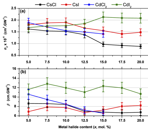
Fig. 7. Evolution of the nonlinear refractive index n_2 (a) and the nonlinear absorption coefficient \beta (b) of glasses as a function of the metal halide content in the glass matrix [\text{GeS}_2]_{0.80}[\text{Ga}_2\text{S}_3]_{0.20} .
