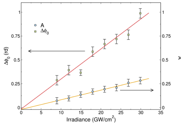
Fig. 2. Dependence of the coefficient A and \Delta\Phi_0 with the irradiance and their linear fit. The slopes of the linear fits are used for the determination of \beta and n_2 .
