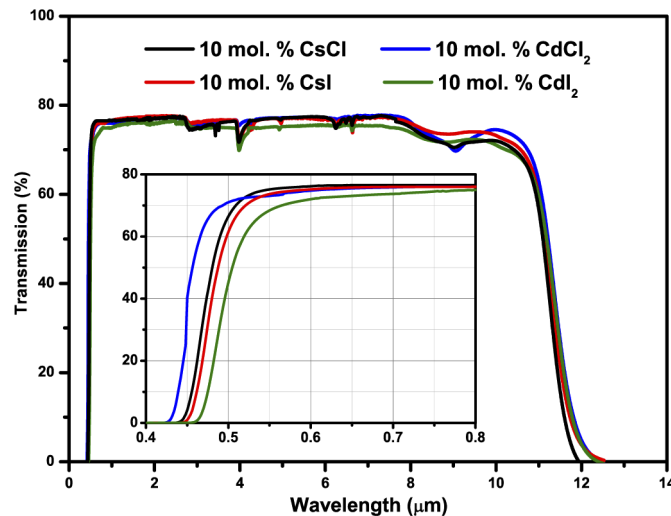
Fig. 5. Vis-IR transmission curves of glass bulks of 1 mm-thickness containing 10% mol. of metal halide. The inset focused on the low-part wavelength to emphasize their visible absorption edge.
