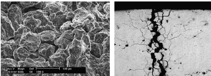
Figure 22.2. Intergranular rupture of the injection nozzle [COA 06]
