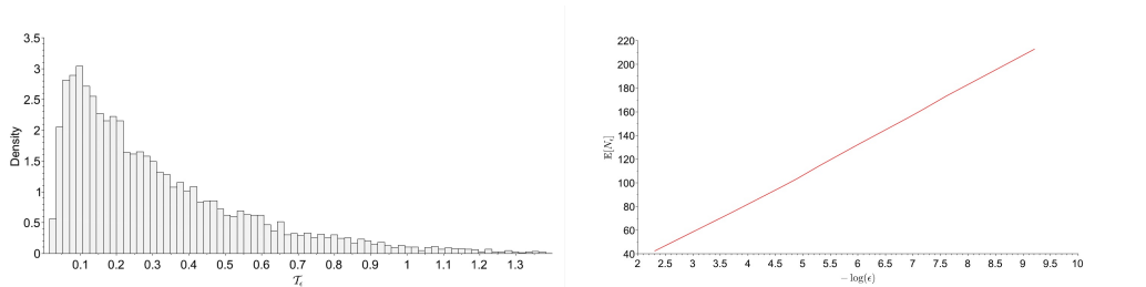
Figure 2: Histogram of the outcome variable for the diffusion (4) with X_0 = 1 , [a, b] = [-1, 2] , \epsilon = 10^{-2} and \gamma = 10^{-4} (left). Average number of steps in ALGORITHM m for the exit time of [-1, 2] (right, in logarithmic scale).
