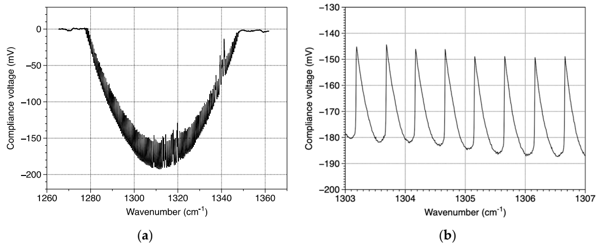
Figure 10. (a) QCL device compliance voltage when varying the mirror angle \pm 3^\circ and (b) a zoom on Figure 10a around 1305\text{ cm}^{-1} .
